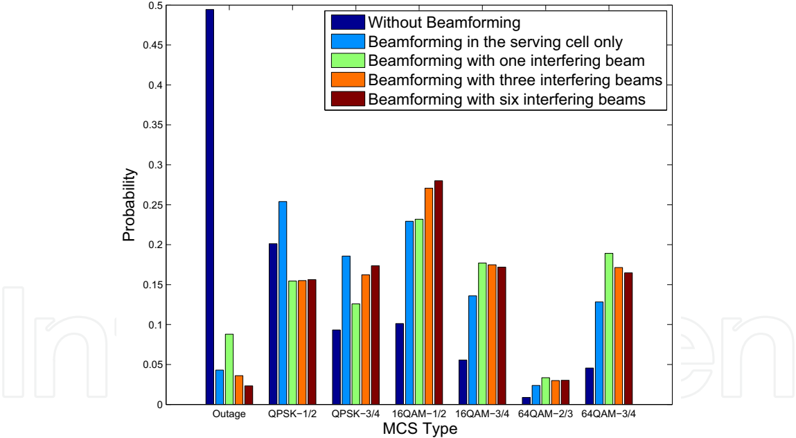
Fig. 6. MCS distribution for PUSC.
