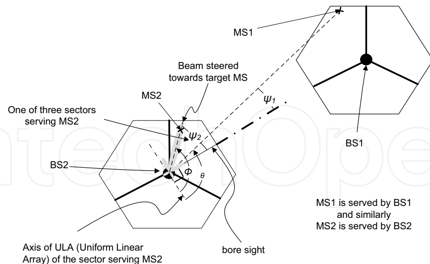
Fig. 3. Example showing beamforming scenario.
