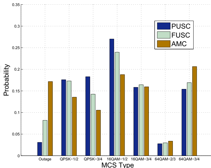
Fig. 9. MCS distribution for PUSC/FUSC/AMC with beamforming.
