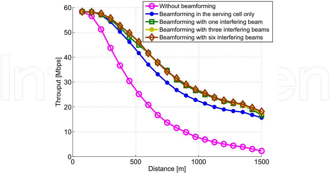
Fig. 5. Average cell throughput versus distance to base station for PUSC.
