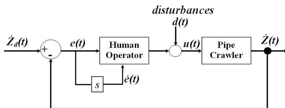
Fig. 5. Closed-loop system of the HITL simulator.
