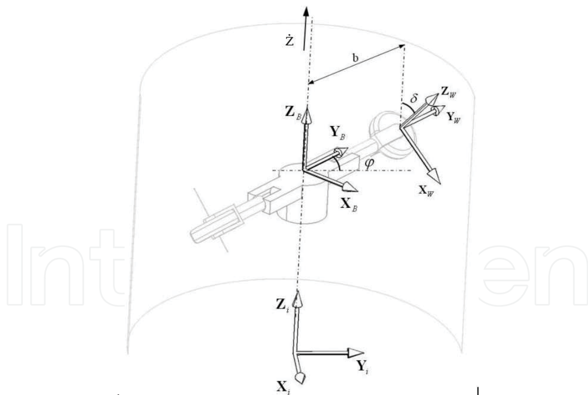
Fig. 3. The simplified model of the robot, with one pair of driving wheels, showing three reference frames. Passive wheels are not shown in this picture.
