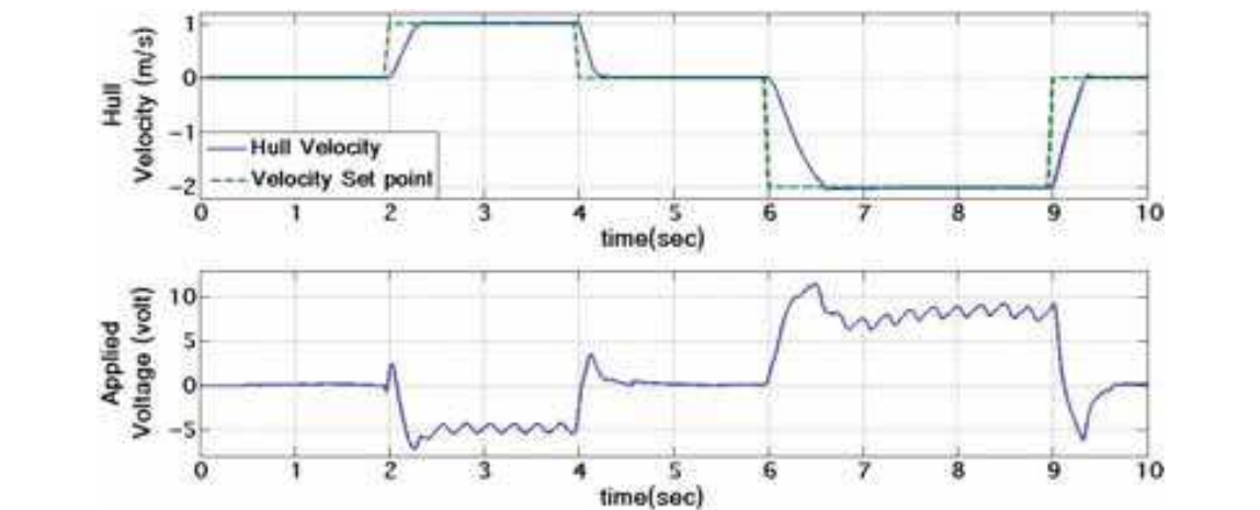
Fig. 30. Experimental results with step reference trajectory of the velocity set point, \dot{Z}_{set} using FLC.
