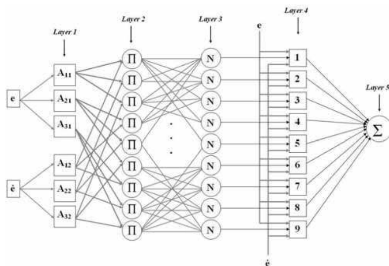
Fig. 9. The ANFIS structure adopted in this work.
