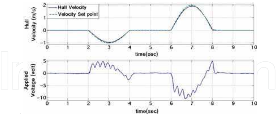
Fig. 29. Experimental results with sinusoidal reference trajectory of the velocity set point, \dot{Z}_{set} using FLC.
