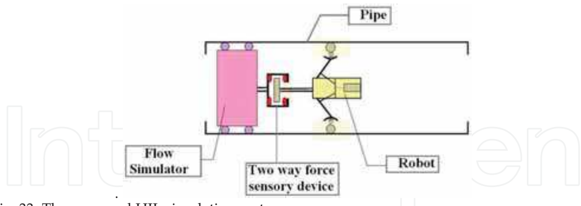
Fig. 33. The proposed HIL simulation system.
