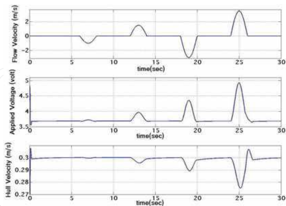
Fig. 25. Response of the closed-loop system with sinusoidal flow disturbance for \dot{Z}_{set} = 0.30 \frac{m}{s} using FLC.
