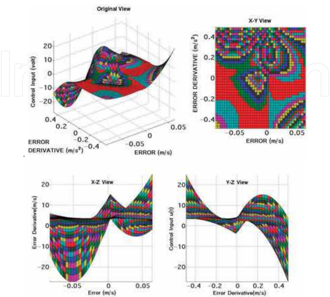
Fig. 22. Control surface of the FLC using three product-of-sigmoidal MF's, four views.
