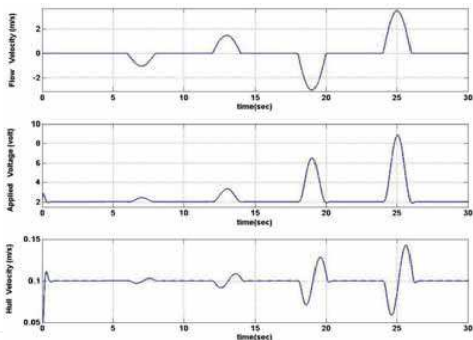
Fig. 12. Response of the closed-loop system with sinusoidal flow disturbance for \dot{Z}_{set} = 0.10 m/s using PID.
