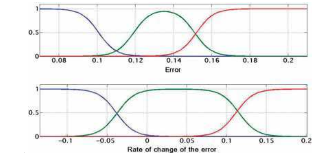
Fig. 21. MF's on the two inputs of the system : error and the rate of change in error, after tuning.
