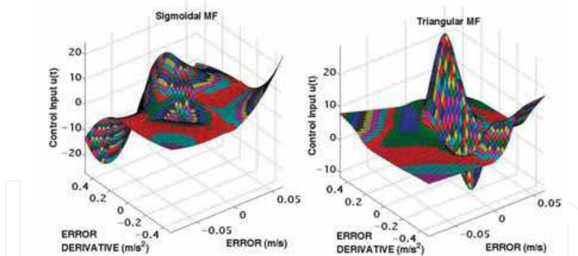
Fig. 31. Comparison between two control surfaces using triangular (left) and sigmoidal MF's (right).
