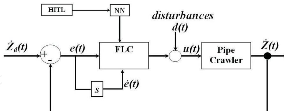
Fig. 6. FLC-based closed-loop system.
