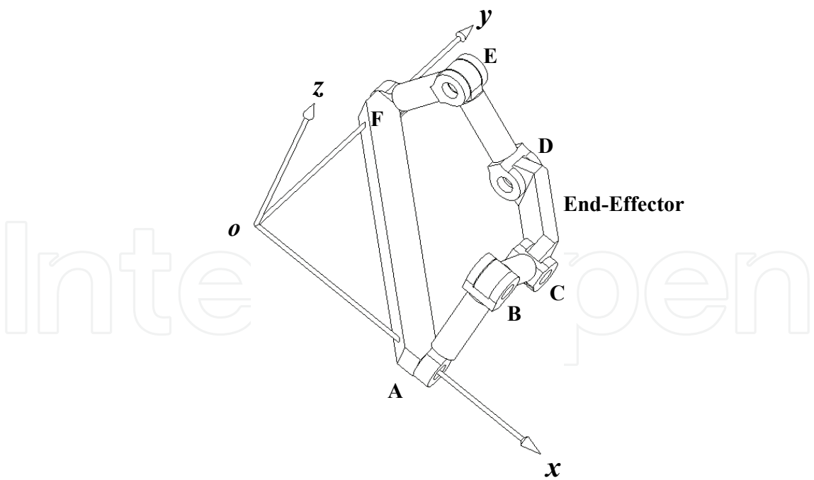
Fig. 11 a Spatial Six-Link Mechanism with the Best Structure Stability The solution of equation (48) is:
