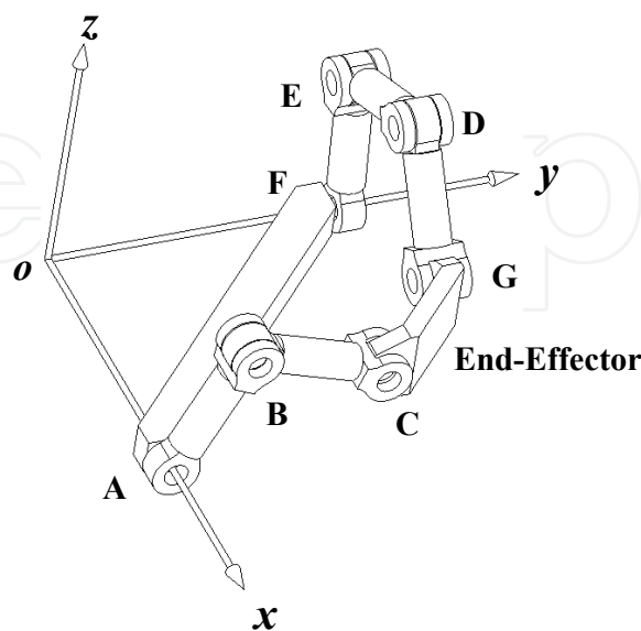
Fig. 13 Configuration of the Spatial Seven-Link Mechanism
