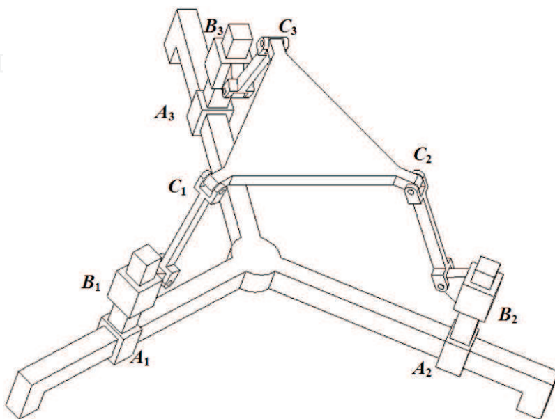
Fig. 1 a 3-PPRR Spatial Mechanism
