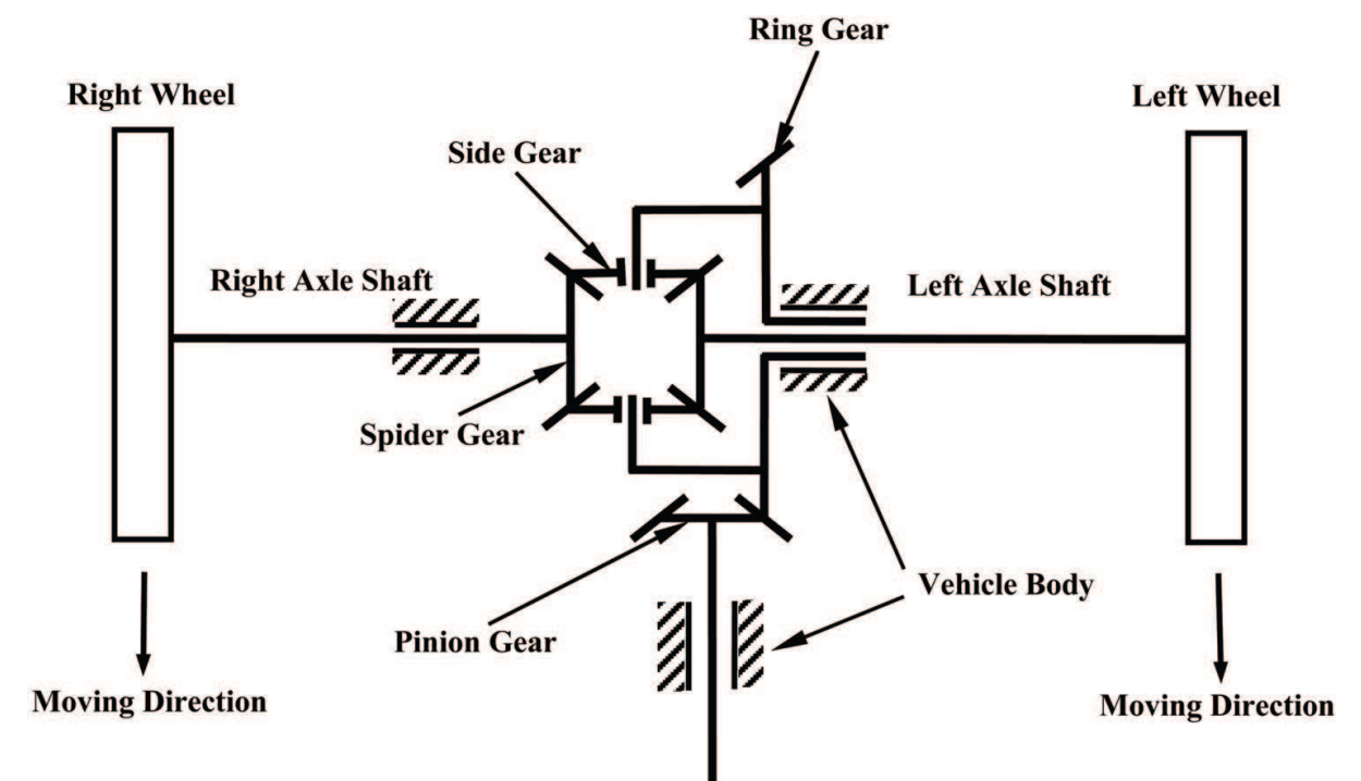
Fig. 3 the differential gear train mechanism
