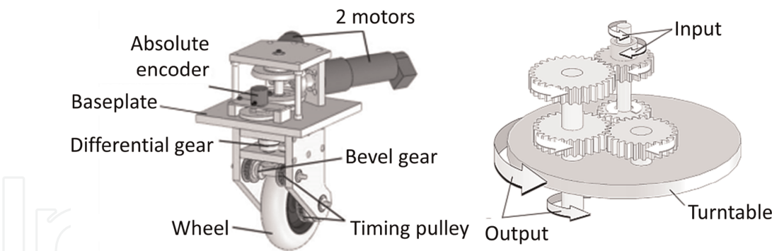
Figure 3. Structural drawing of the DDSS developed by the authors, an omni-directional wheel that maximizes the efficiency of two motors and can move instantly in any direction.
