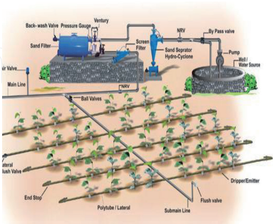
Figure 1. Simple Drip irrigation Model.
