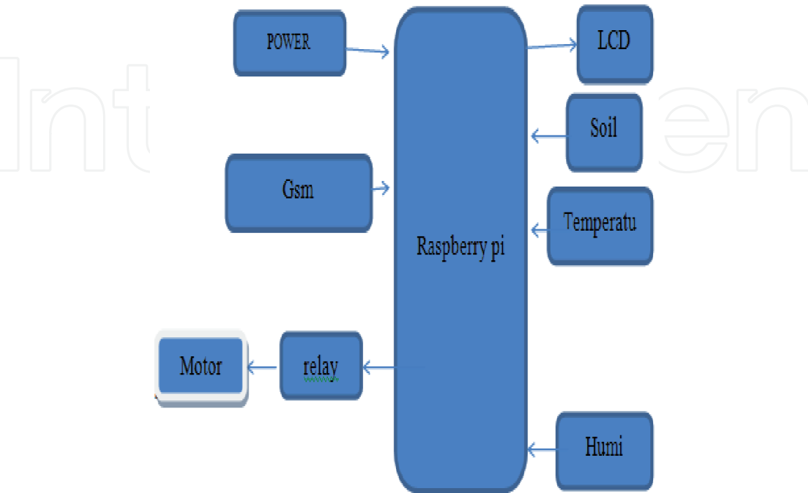
Figure 4. Smart Irrigation with Raspberry Pi and GSM.
