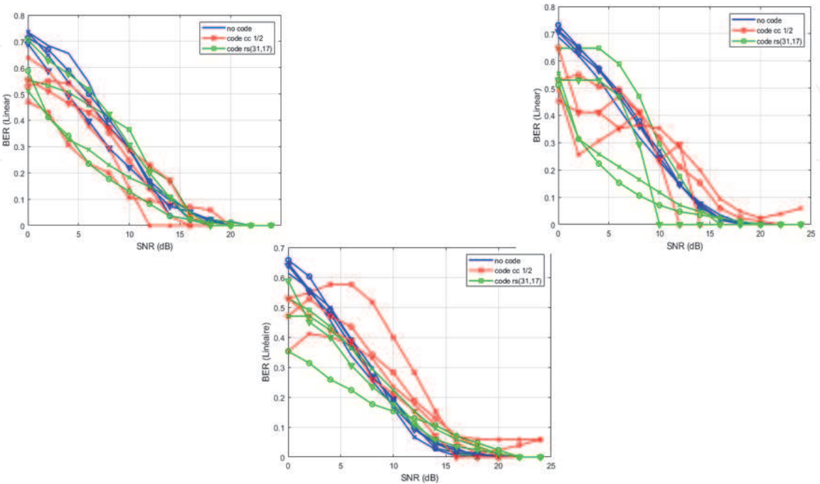
Figure 19. BER/SNR on a fading channel with AWGN noise for MTO mode.
