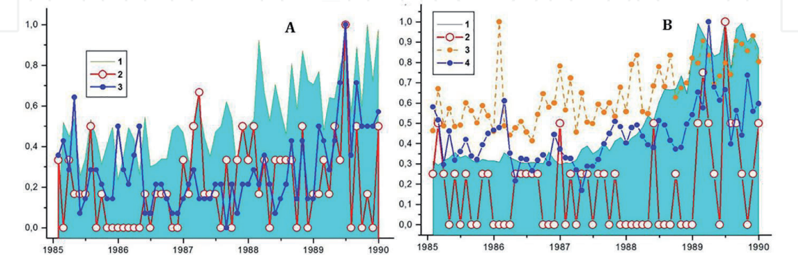
Figure 2. Coherent dynamics of the average monthly values of the parameters of geocosmic agents and the monthly values of morbidity. A. Parameter of solar wind “sigma-phi-V, deg” (1, graph area—cyan), the incidence of the mental MD (2), incidence of the injuries and poisoning on the way to and from work, IP (3). B. Solar radio emission with wavelength 10.7 cm (1, graph area—cyan), incidence of the diseases of arteries, arterioles, and veins (2), sigma-theta-V, deg. (3), pc (N) index (4). X axis: The months of the year from January 1985 to December 1989; Y axis: the normalized values of the all parameters.
