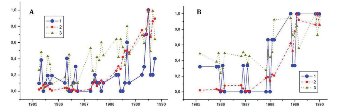
Figure 6. The stable links between injury rates and poisoning on the way to work and from work with similar geocosmic agents during the polar day (A) and the polar night (B). A, B. Dynamics of the monthly values of incidence of the injury and poisoning on the way to work and from work (1), the monthly average magnitudes of the solar radio emission with wavelength 10.7 cm (2), and the solar wind parameter “sigma-phi-V”(3). X axis: the months from January 1985 to December 1989, where months from March to September are included in the period of the polar day (A); the months from October to February are included in the period of the polar night (B); Y axis: all normalized parameters.
