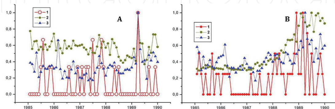
Figure 3. Coherency dynamics of the monthly values of morbidity and the monthly average values of the parameters of geocsmic agents. A. Incidences of the complications of pregnancy and the postpartum period, CPP (1); flow pressure of the solar wind, (nPa) (2); and ap-index (3). B. Incidences of the inflammatory processes of the female pelvic organs and other diseases of the female genital organs, IFGO(1), the solar radio emission with wavelength 10.7 cm (2), PC(N)-index. X axis: the months of the year from January 1985 to December 1989; Y axis: the normalized values of the all parameters.
