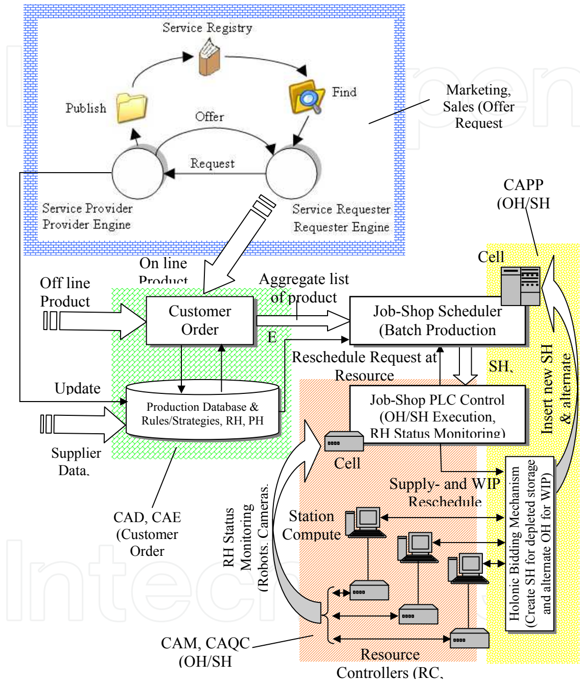
Fig. 7. Information and data flow of HMES with knowledge-based Service Oriented Architecture for customer request management
