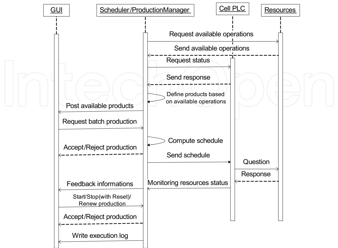
Fig. 8. Time diagram representing messages exchanged between entities from the business domain
