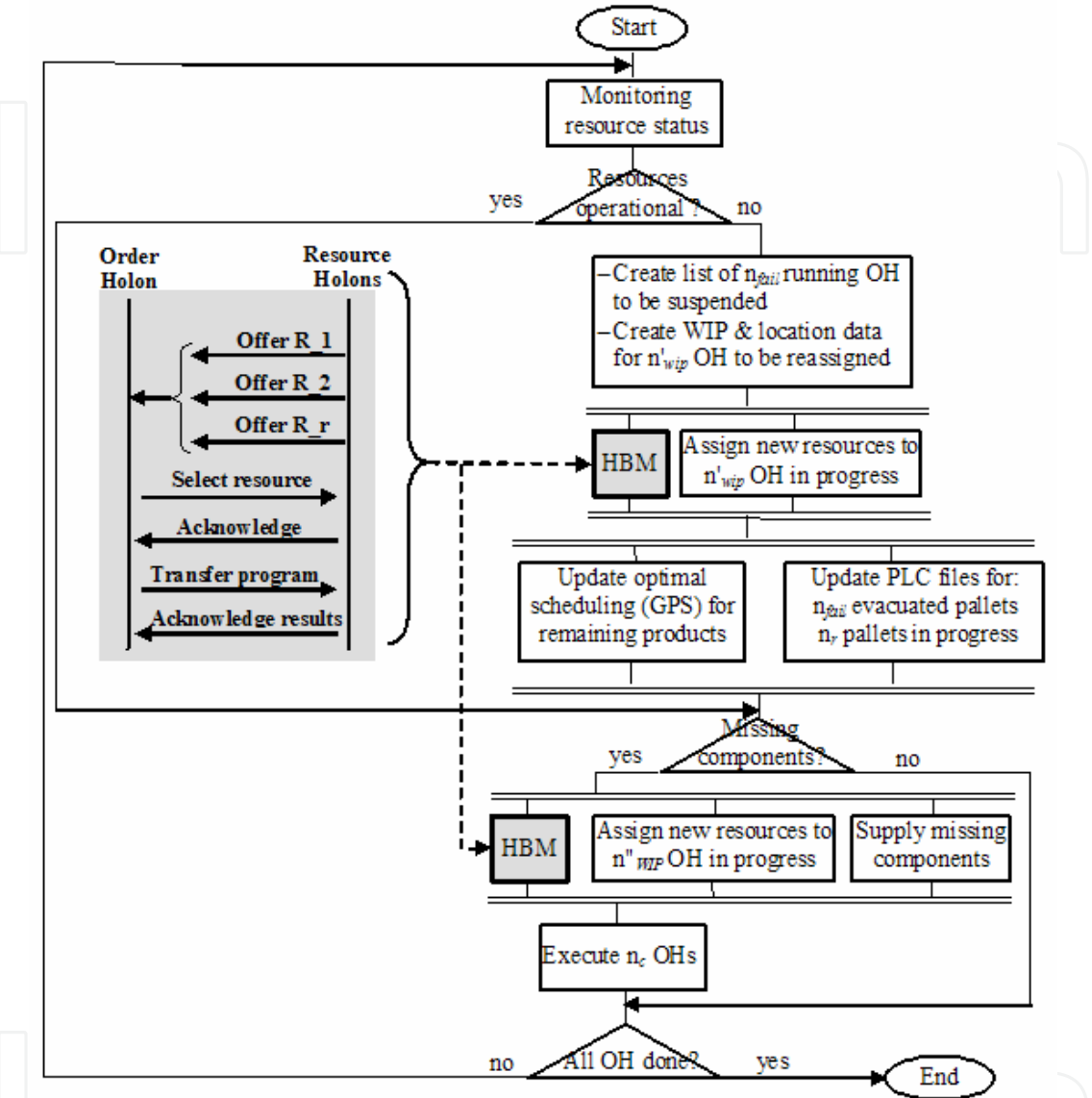
Fig. 14. Dynamic OH rescheduling at resource failure/storage depletion with embedded CNP job negotiation
