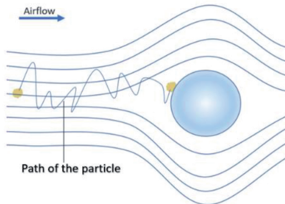
Figure 4. Model of diffusion mechanism, depends on the motion of the particle causing contact with a fiber.
