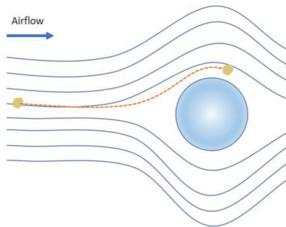
Figure 3. Model of interception effect mechanism, depends on the collision between the fiber and the particle passing through the filter.
