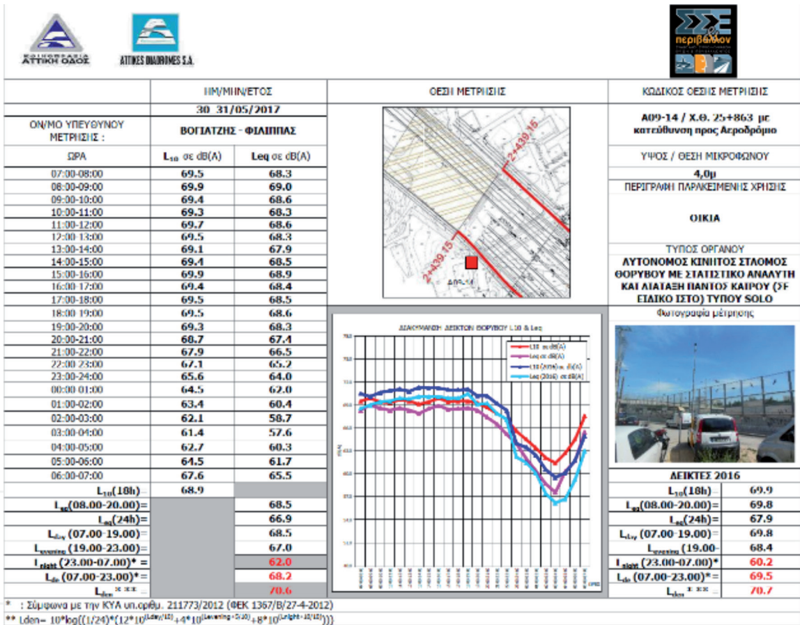
Figure 2. A typical 24-h measurement in Athens Ring Road (2017) (accessed in three periods: day, evening, and night).
