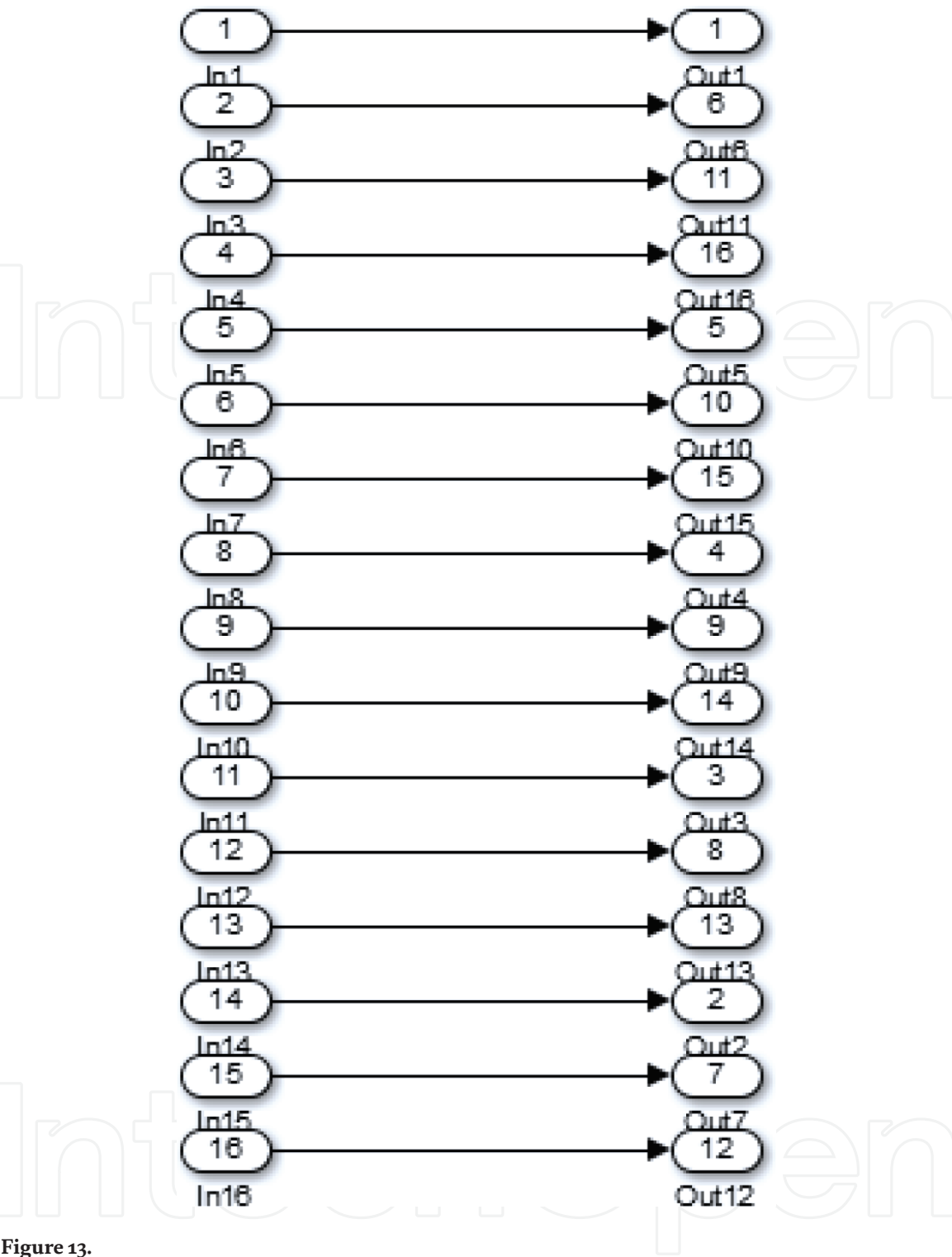
Figure 13. Implementation of shift row.
