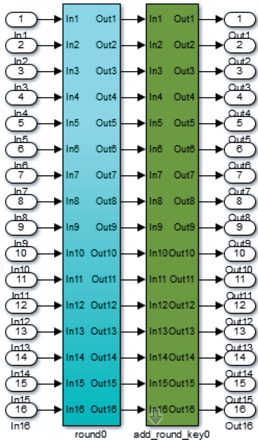
Figure 10. System generator-based model of round function.
