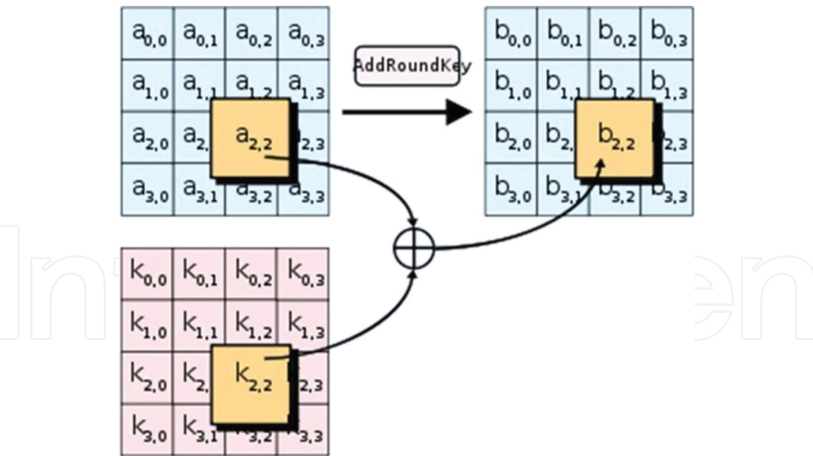
Figure 6. Add round key stage.
