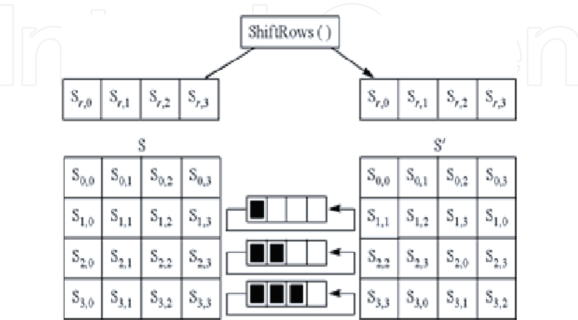
Figure 4. Shift row stage.
