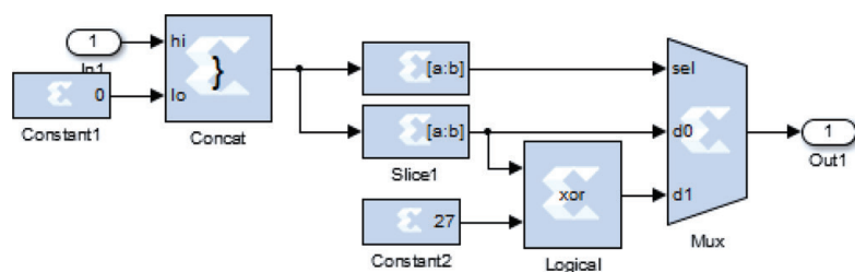
Figure 22. Implementation of multipliers.
