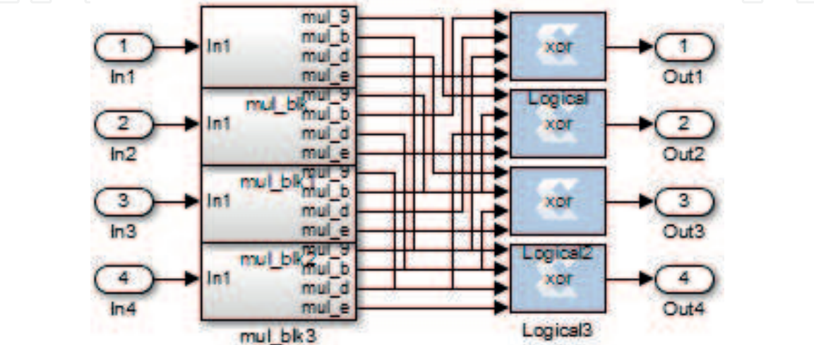
Figure 20. Implementation of group.
