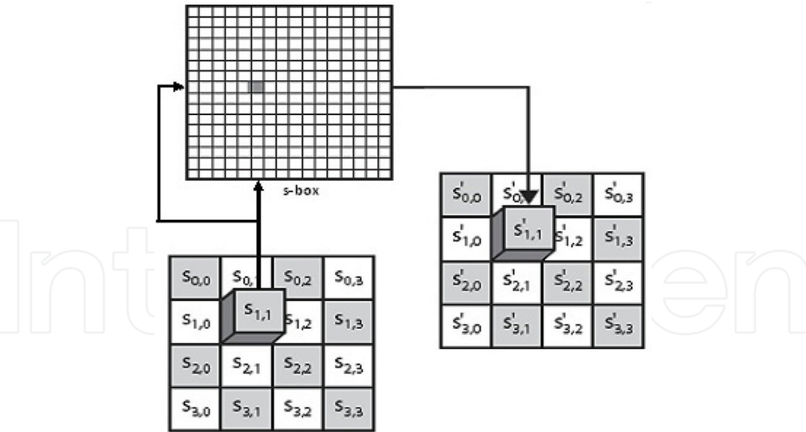
Figure 3. Byte substitution stage.
