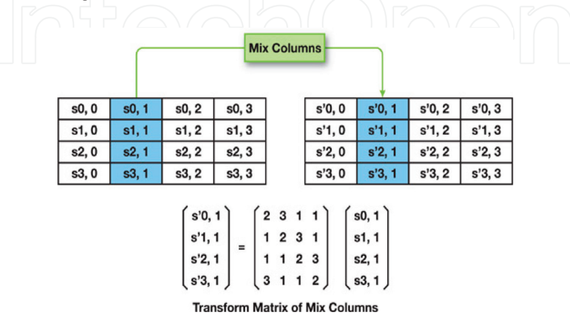
Figure 5. Mix column stage.
