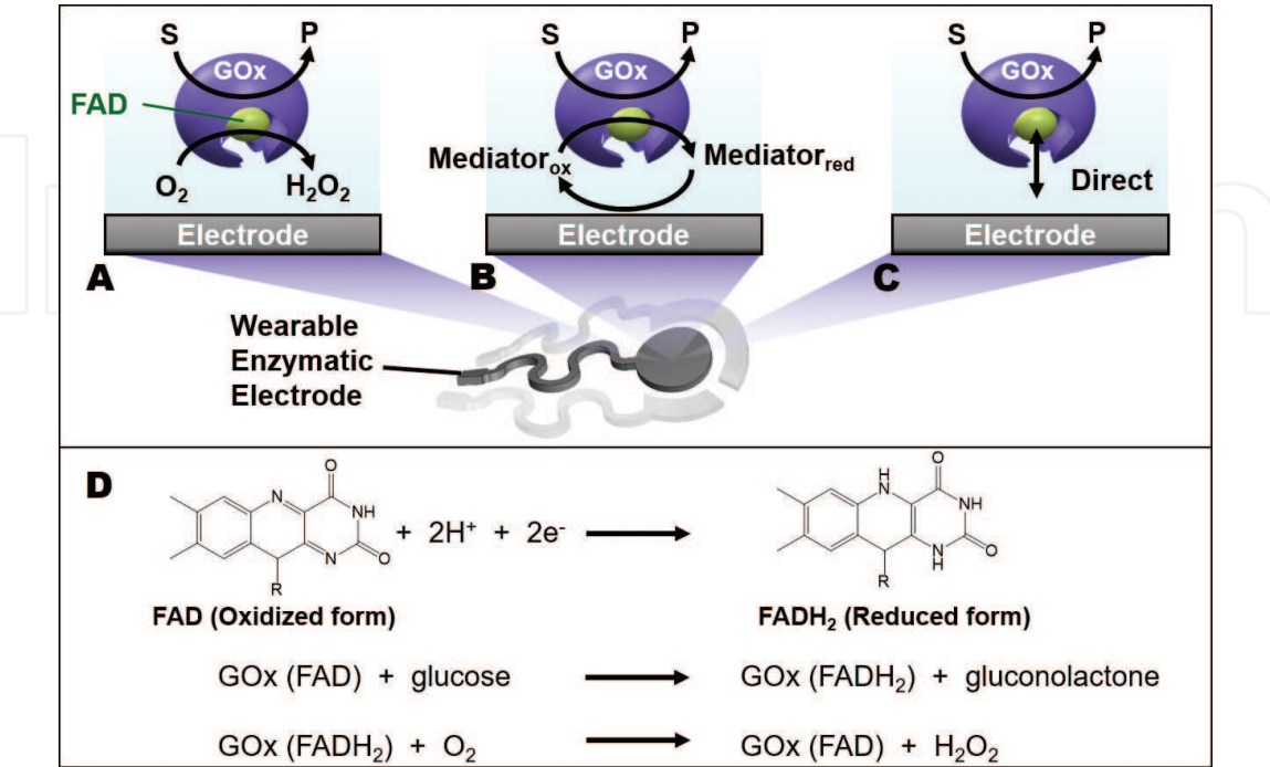
Figure 4. Principles of interfacing the enzyme, such as glucose oxidase (GOx), with the electrode. Different generations of strategies (A–C: first, second, and third generations) are illustrated. (D) Reactions involving the glucose oxidase biocatalyst.
