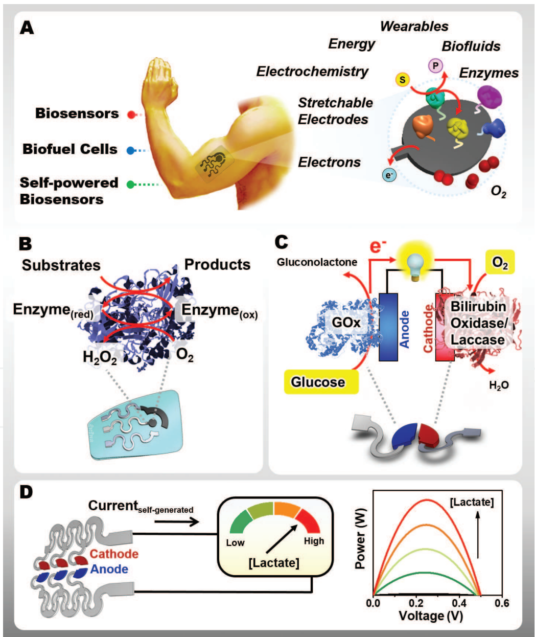
Figure 1. (A) Skin-worn enzyme-based electrochemical devices. The soft electrode platform is functionalized with enzymes, allowing various applications, including (B) biosensors, (C) energy-harvesting biofuel cells, and (D) self-powered biosensors.
