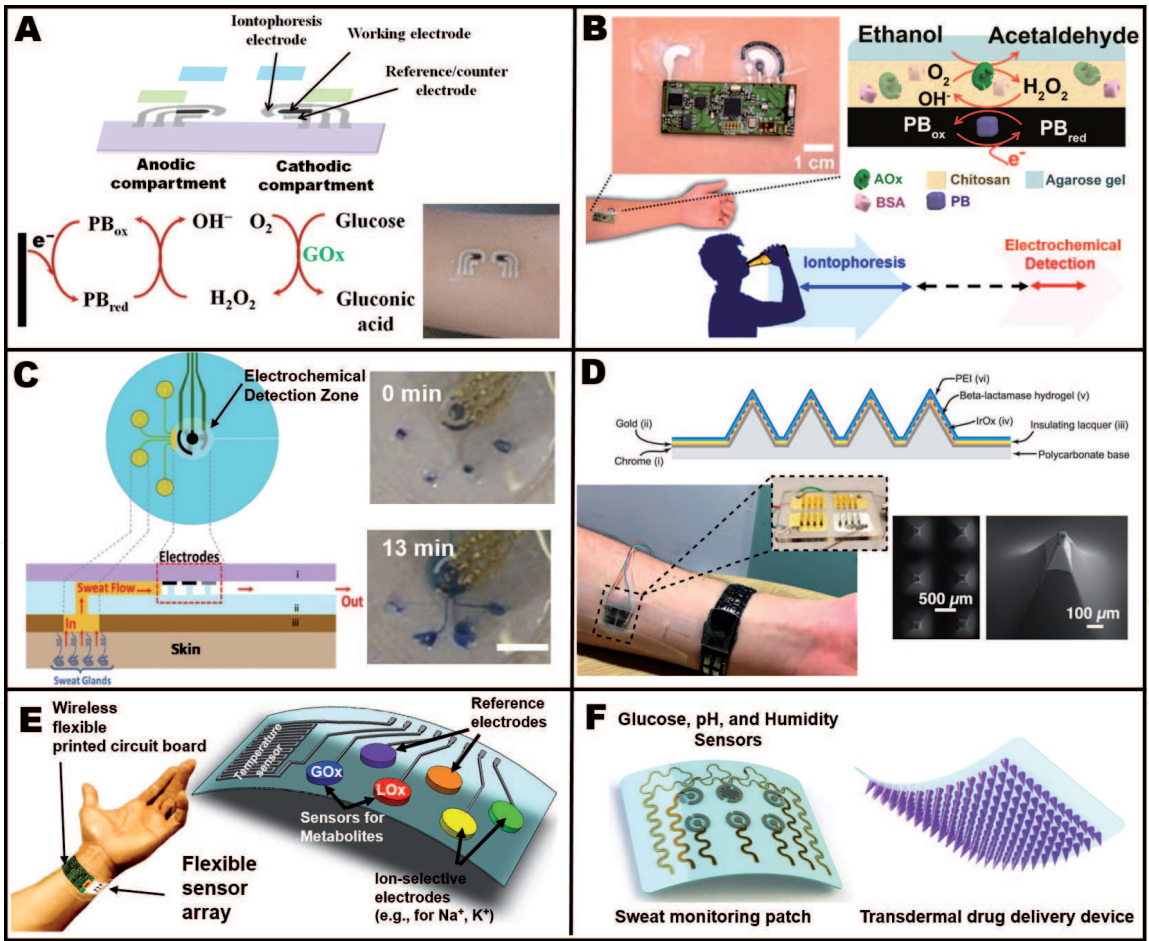
Figure 2. Skin-worn enzyme-based electrochemical biosensors. (A) Transdermal tattoo-based glucose sensors, coupled with reversed iontophoresis [17]. Adapted with permission from ref [17]. Copyright 2015 American Chemical Society. (B) Tattoo-based alcohol biosensors, coupled with pilocarpine iontophoresis and wireless electronics [18]. Adapted with permission from ref [18]. Copyright 2016 American Chemical Society. (C) Biosensors integrated with a microfluidic patch for sweat collection and analysis [20]. Adapted with permission from ref [20]. Copyright 2017 American Chemical Society. (D) Microneedle-based β-lactam sensors [22]. Adapted with permission from ref [22]. Copyright 2019 American Chemical Society. (E) Integrated glucose/lactate enzymatic biosensors with electrolyte and temperature sensors. (F) Integrated sweat monitoring biosensing and transdermal drug delivery system.
