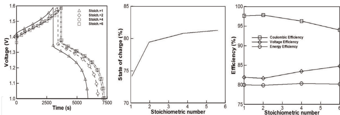
Figure 7. Current density of 75 \text{ mA/cm}^2 at various flow rates; (a) charge–discharge curve, (b) SOC, and (c) efficiencies as a function of stoichiometric number ( \lambda = Q_{\text{real}} / Q_{\text{theo}} ). Reproduced with permission from [8]. Copyright 2018 Elsevier.
