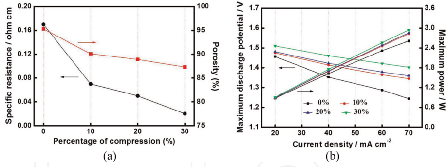
Figure 6. (a) Specific resistance and porosity vs. percentage of compression for FA-30A carbon felt electrodes and (b) polarization curves of VRFB cells with electrodes of various levels of compression. Reproduced with permission from [21]. Copyright 2014 Elsevier.
