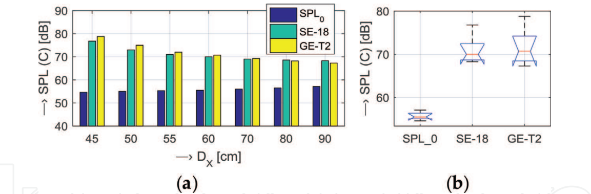
Figure 10. Mapping of the acoustic noise SPL at different distances D_x = \{45, 50, 55, 60, 70, 80, 90\} cm from the middle of the scanning area of the MRI device for SE/GE sequences: (a) comparison of the SPL values with those of the background noise ( SPL_0 ) and (b) box-plot of their basic statistical parameters.
