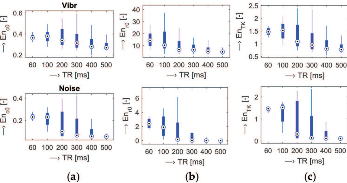
Figure 12. Visualization of energetic relations of the vibration (upper set of graphs) and noise (lower set) signals for different TR times; {60, 100, 200, 300, 400, 500} ms—basic statistical parameters of: (a) En_{co} , (b) En_{ro} , and (c) En_{TK} ; used Hi-Res GE-T2 sequences with TE = 22 ms and sagittal orientation.
