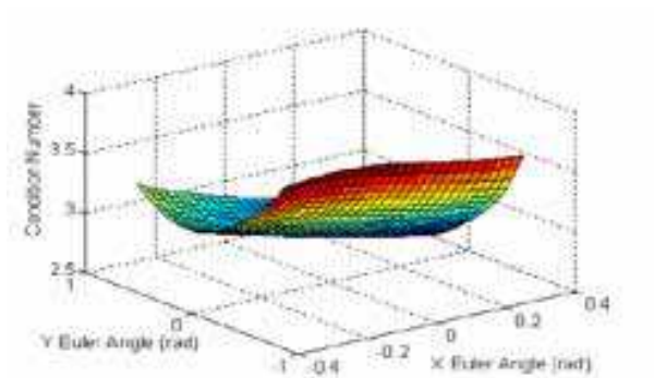
Fig. 9. Condition number vs. orientation at \phi = 20^\circ
