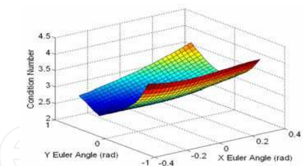
Fig. 8. Condition number vs. orientation at ( \phi = -20^\circ )
