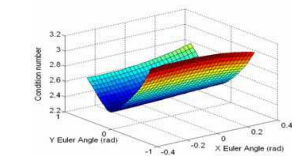
Fig. 10. Condition number vs. orientation at ( \phi = 0^\circ )
