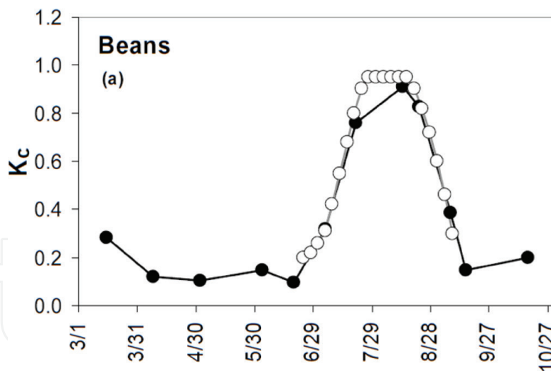
Figure 1. Constructed K_c (or ET_rF ) curve for a bean crop from METRIC (dark symbols) with comparison against a standard K_c curve produced by the US Bureau of Reclamation Agrimet service for a region near Twin Falls, Idaho in year 2000.
