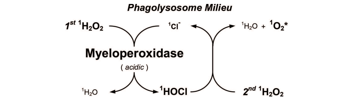
Figure 3. Schema depicting myeloperoxidase-catalyzed \text{H}_2\text{O}_2 -dependent oxidation of chloride to hypochlorite, and its reaction with a second \text{H}_2\text{O}_2 to generate ^1\text{O}_2^* . The spin multiplicity of each molecule is indicated by the superscripted number preceding the molecular description.
