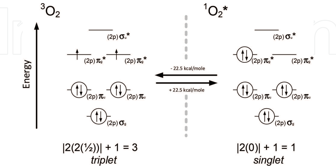
Figure 1. Triplet and electronically excited singlet molecular oxygen with emphasis on the \pi^* (pi antibonding) frontier orbitals. The two \pi^* are degenerate (same energy level). Hund's maximum multiplicity rule predicts lowest energy is achieved when each SOMO electron has the same spin, that is, the triplet state ( ^3\text{O}_2 ). The electronic energy of ^1\text{O}_2^* is 22.5 kcal/mol (94.2 kJ/mol) above ^3\text{O}_2 .
