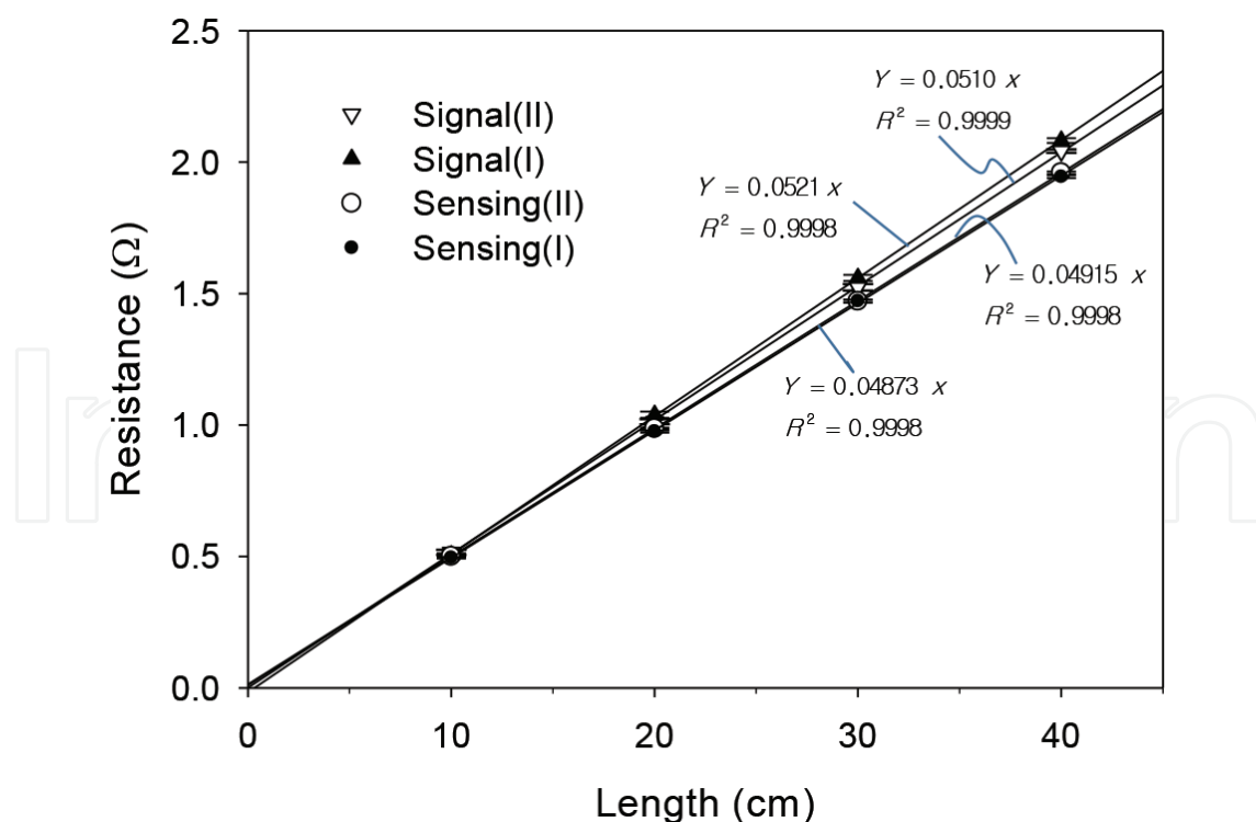
Figure 3. Electrical resistance linearity of four MCEYs as a function of the yarn length.
