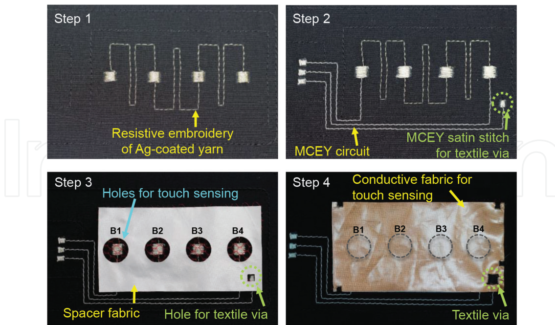
Figure 5. A one-stop production process on a standard CNC embroidery machine for fabricating the multilayer structured textile touch sensor that senses a touched position [16].
