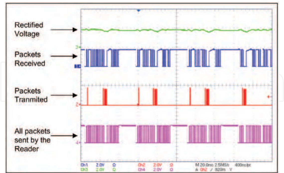
Fig. 6. Scope plot of the WISP responding to EPC queries along with the its rectified voltage.
