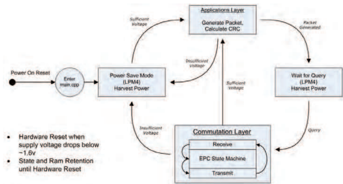
Fig. 5. Power Management Algorithm
