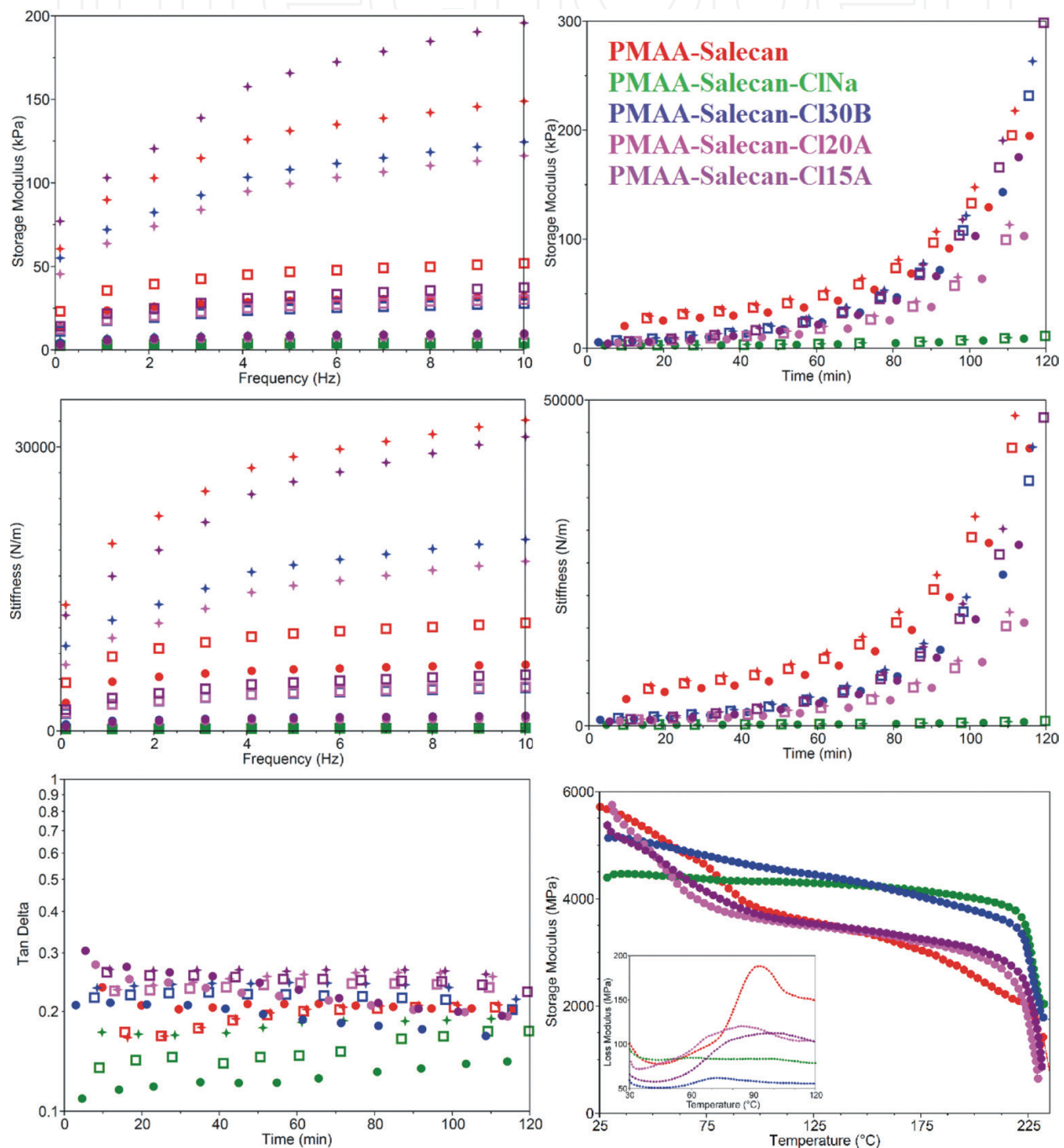
Figure 9. DMA results: storage modulus as a function of frequency and time; stiffness as a function of frequency and time; Tan Delta as a function of time; storage modulus as a function of temperature for: PMAA-Salecan; PMAA-Salecan-CINa; PMAA-Salecan-CI30B; PMAA-Salecan-CI20A; and PMAA-Salecan-CI15A.
