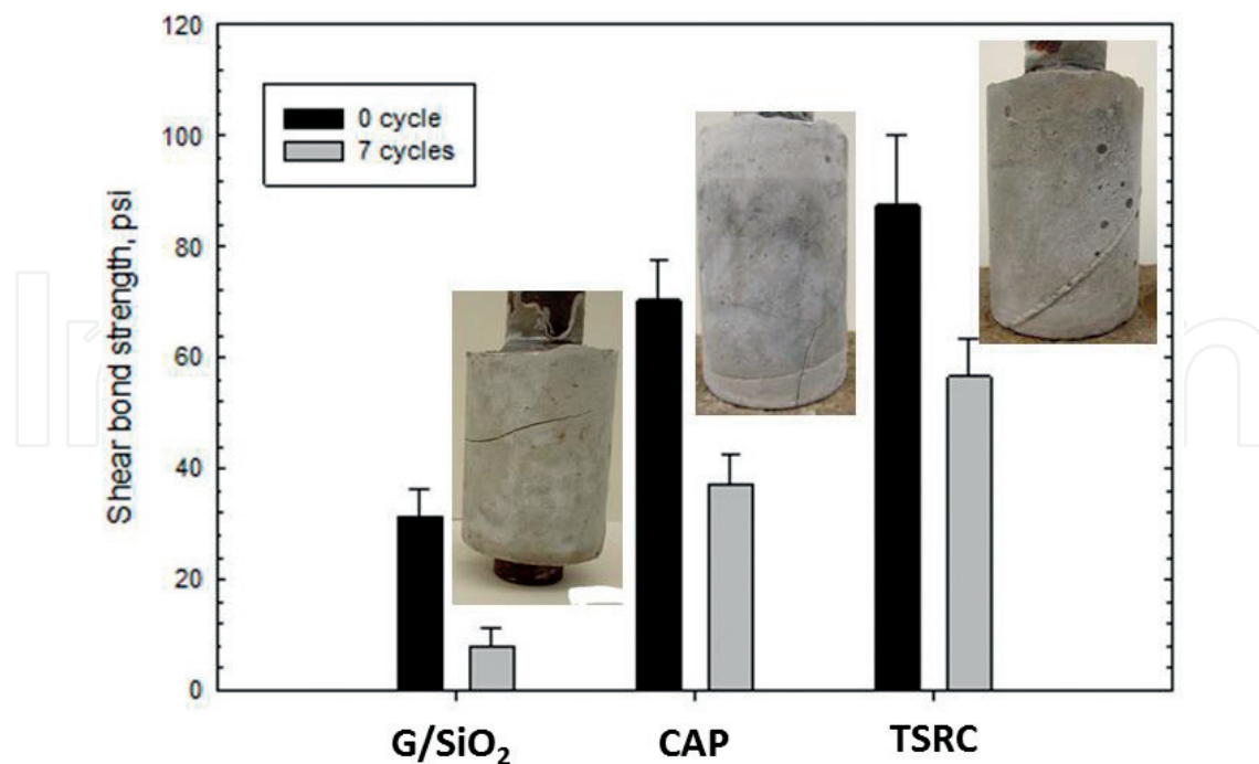
Figure 1. Shear bond strength and appearance of cement-CS sheath samples hydrothermally cured at 300°C and subjected to 7 cycles of thermal shock tests.
