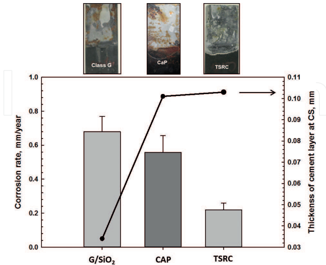
Figure 2. Corrosion rate, cement layer thickness and appearance of carbon steel samples with cement layer after hydrothermal curing for total 6 d at 300°C.
