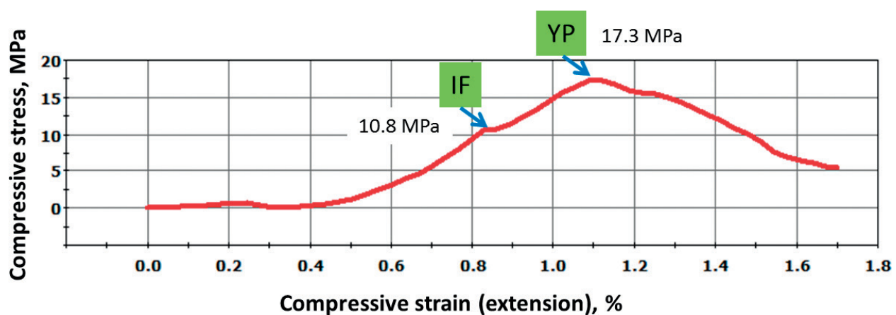
Figure 4. Strain–stress compressive curve for TSRC sample broken into two pieces and re-bonded in alkali carbonate (0.05 M NaCO 3 ) at 300°C for 5 days; points of breaking off the re-adhered piece (initial failure, IF) and the yield point (YP) of the sample are shown.
