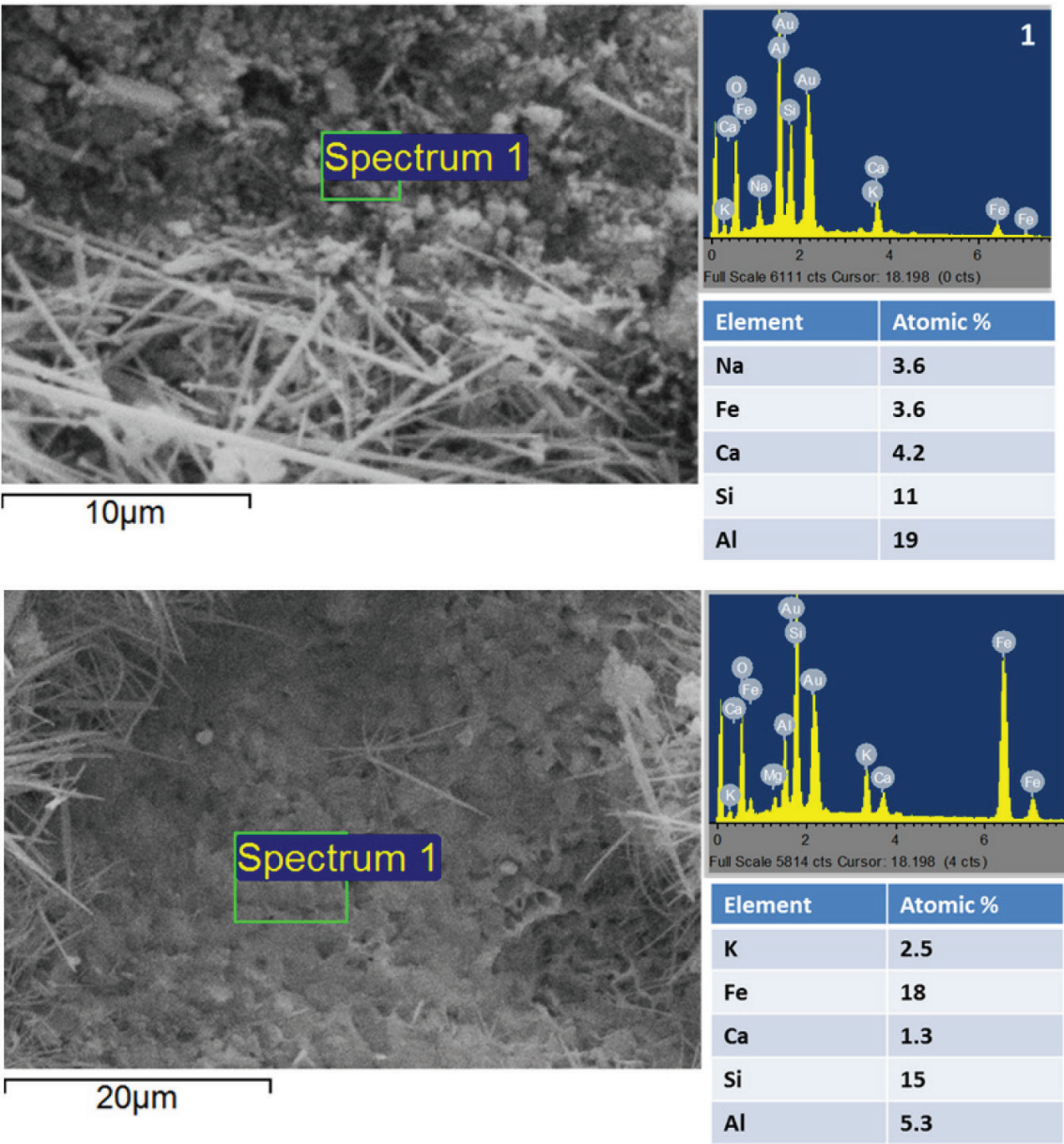
Figure 3. Microphotographs and elemental compositions of TSRC (top) and G/SiO 2 layers on carbon steel plates after 6 d hydrothermal curing at 300°C.
