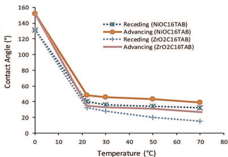
Figure 3. \theta_R and \theta_A depicting wettability change of NiO, ZrO 2 (0.05 wt.%), C 16 TAB (0.5 wt.%) blends in toluene (1-hour Exposure time) at different temperatures [24] ® .
