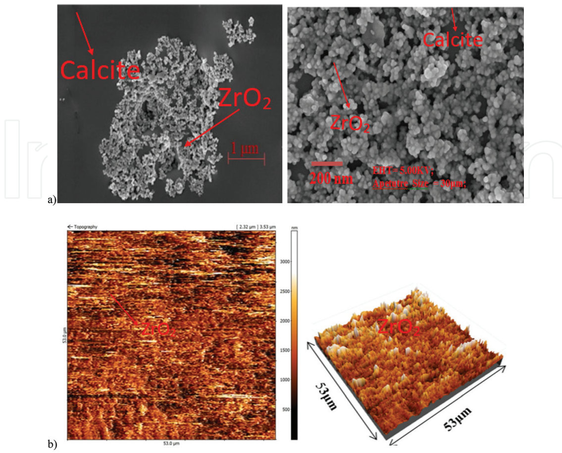
Figure 5. SEM (a) and AFM(b) images of \text{ZrO}_2 nanoparticle as uniform nano-spherical particle with mean particle size of 28 nm depicting surface adsorption on calcite substrates [23] © .
