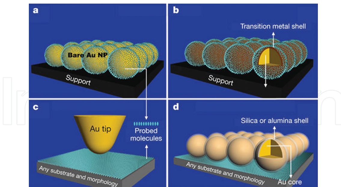
Figure 5. Working mechanism of four types of SERS substrates where small dots represent the probed molecules. (a) Bare Au nanoparticles with probed molecules directly adsorbed to their surfaces, (b) Au core and transition metal shell nanoparticles with probed molecules directly adsorbed to the shell surface, (c) Au tip enhanced Raman probe in non-contact mode and (d) SHINERS: shell-isolated mode preventing the direct contact of the plasmonic core with the probed molecules. Reprinted by permission from Macmillan Publishers Ltd.: Nature Letters [30], copyright 2010.
