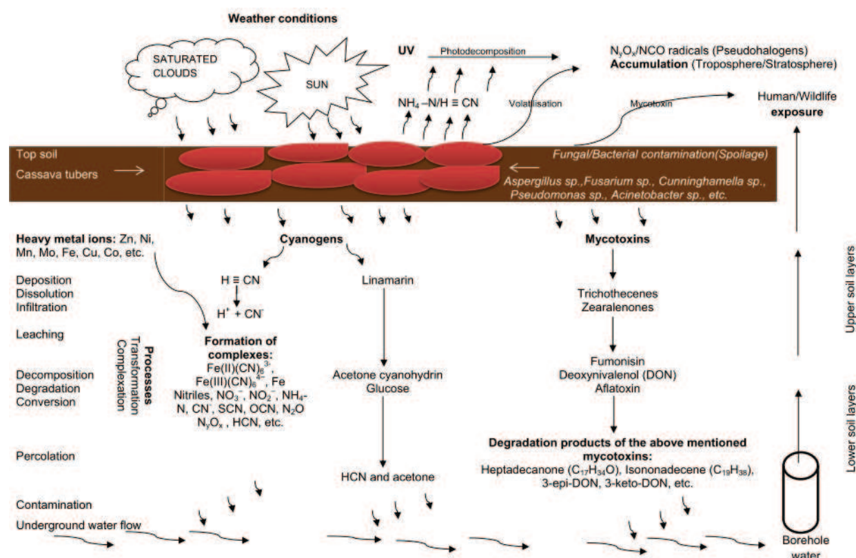
Figure 2. Cassava cyanogen and mycotoxin movement in agricultural soil. Key: \text{NO}_3^- (nitrate), \text{NO}_2^- (nitrite), \text{Fe(II)(CN)}_6^{3-} (ferrocyanide), \text{Fe(III)(CN)}_6^{3-} (ferricyanide), \text{SCN} (thiocyanide), \text{NH}_4\text{-N} (ammonium nitrogen), \text{CN}^- (cyanide ion), \text{-OCN} (cyanate), \text{N}_2\text{O} (nitrous oxide) and \text{N}_y\text{O}_x (nitrogen oxides).
