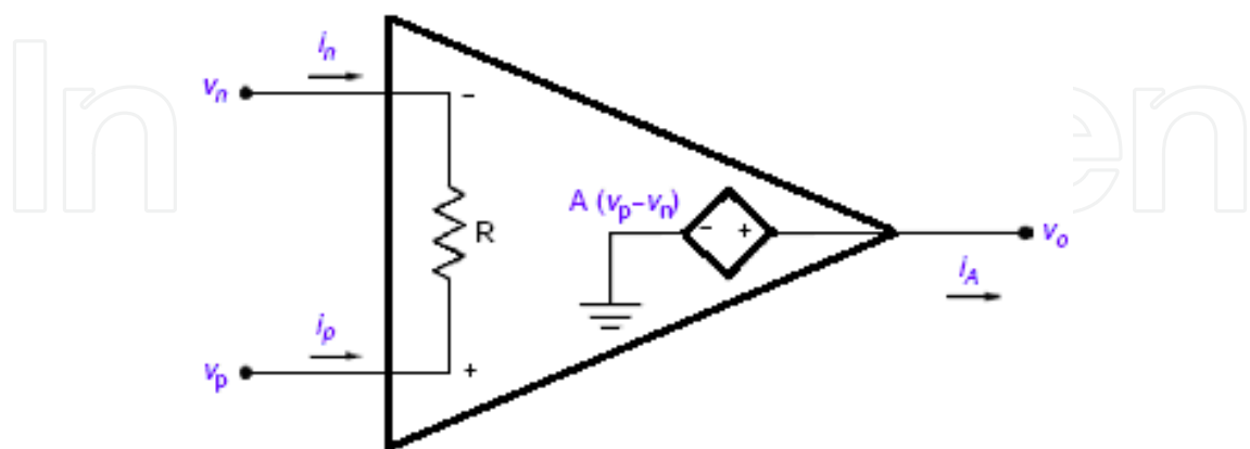
Figure 33. An internal mode of the op amp
