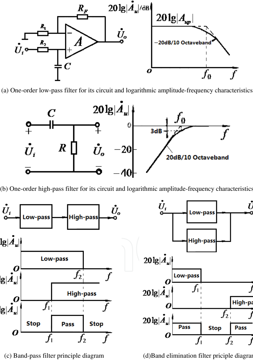
Figure 31. Four types of filters and its amplitude-frequency characteristics
