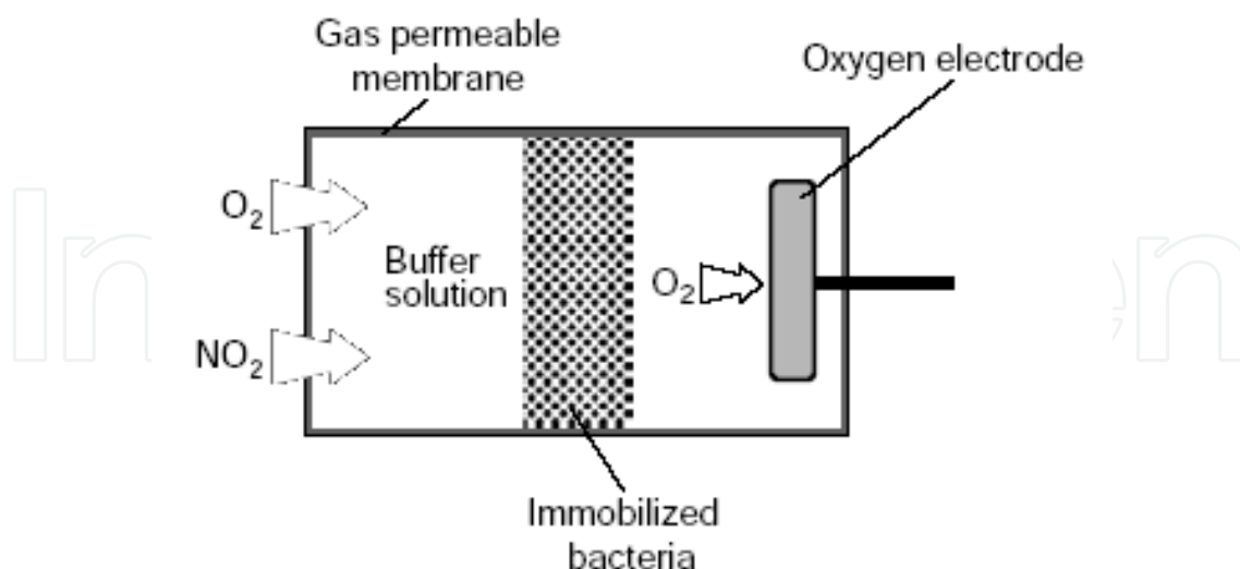
Figure 16. Sensing principle of a \text{NO}_2 microbial biosensor
