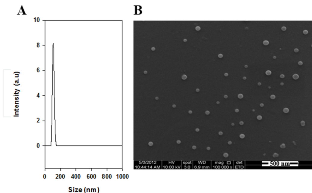
Figure 5. Hydrodynamic size histogram (A) and SEM image (B) of Prot8 particles.
