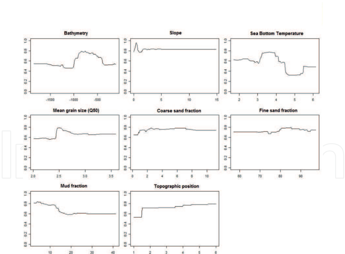
Figure 6. Partial dependence plots showing quantitative influence from each environmental variable on the occurrence of benthic vulnerable organisms predicted probability.
