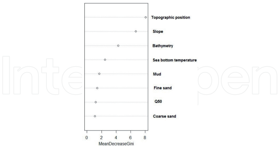
Figure 5. Mean Decrease Gini for each explanatory variable in the RF model. Higher values in the X axis indicate higher influence of the environmental variable on the occurrence of benthic vulnerable organisms.
