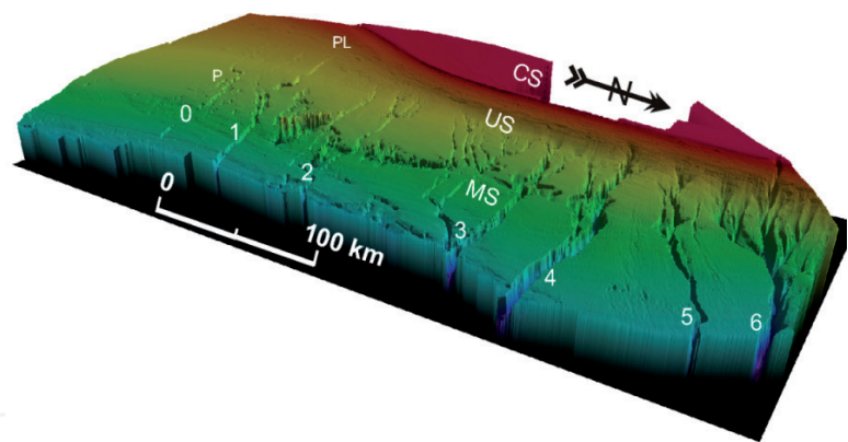
Figure 2. Colour shaded 3D bathymetric map of a segment of the Patagonian Argentinian margin compiled from multi-beam backscatter data. Arabic numbers identify submarine canyons discussed in text. CS=Continental shelf; US=Upper continental slope; MS=Middle continental slope; P=Pockmark; PL=Iceberg plough marks.
