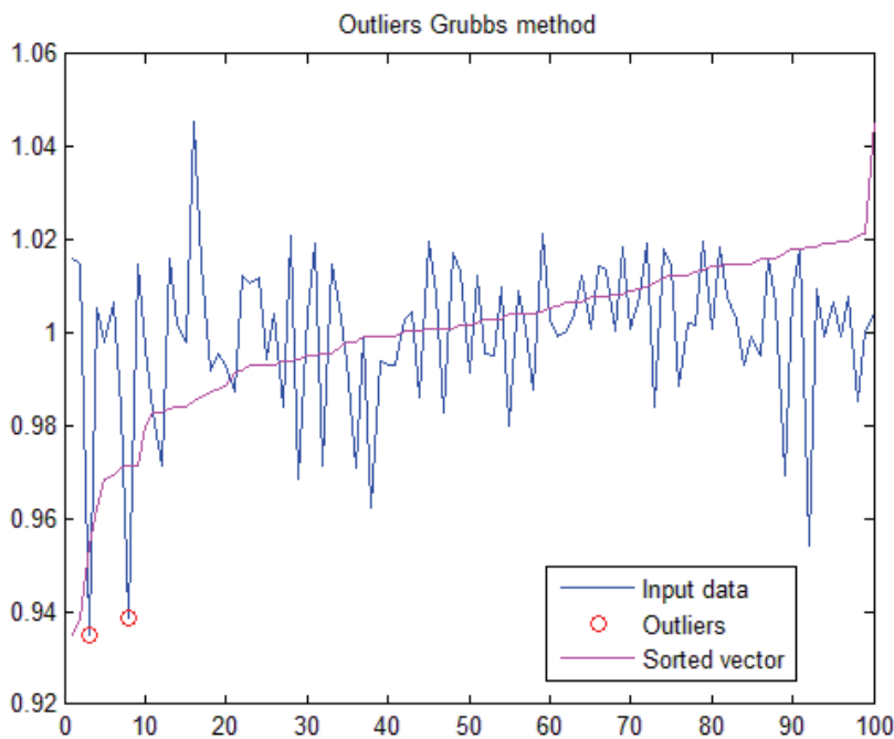
Fig. 2. First example using Grubbs method.
