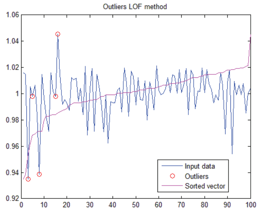
Fig. 3. First example using Local Outlier Factor method.
