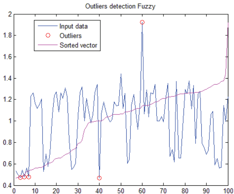
Fig. 7. Second example using Fuzzy Logic method.
