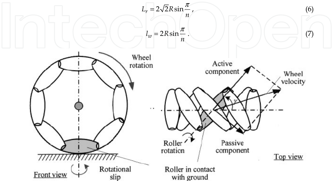
Figure 13. DOFs in a Mecanum wheel [Song & Byun, 2004]
