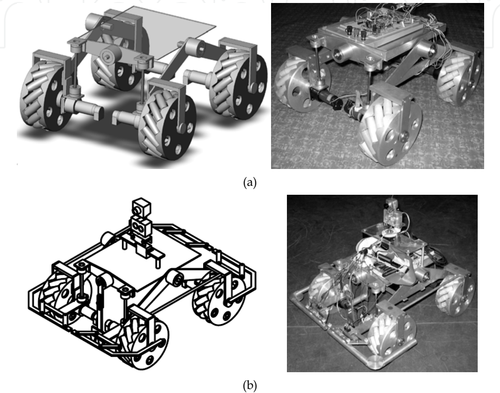
Figure 14. Omnidirectional robot: (a) CAD design and photo of the first prototype; (b) the second prototype
