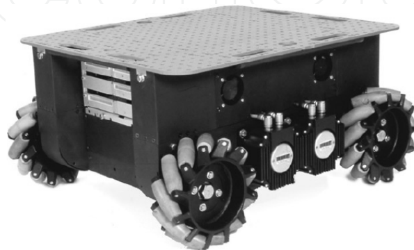
Figure 1. Uranus omnidirectional mobile robot [Muir & Neuman, 1987]
