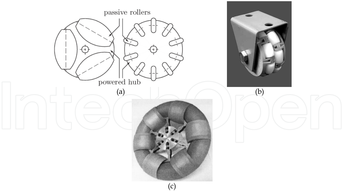
Figure 6. Universal wheel: (a) simple; (b) double; (c) alternate
