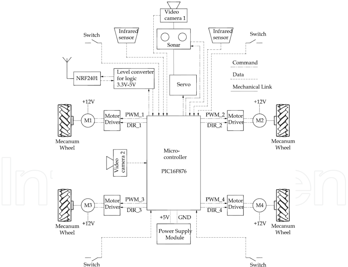
Figure 19. Electronic board
