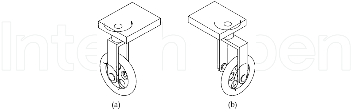
Figure 5. Steered wheel: (a) powered steering wheel; (b) lateral offset
