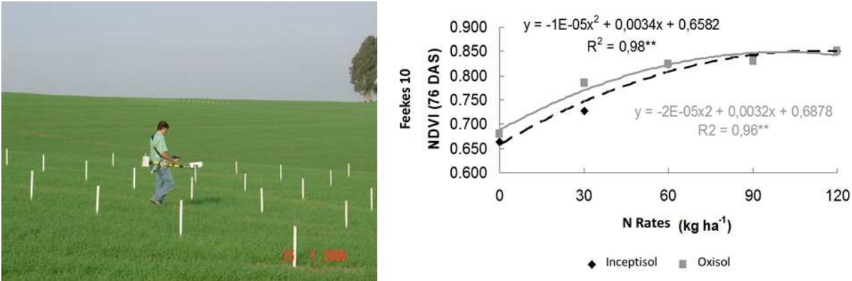
Figure 3. First experiment and NDVI response with nitrogen rates in wheat.
