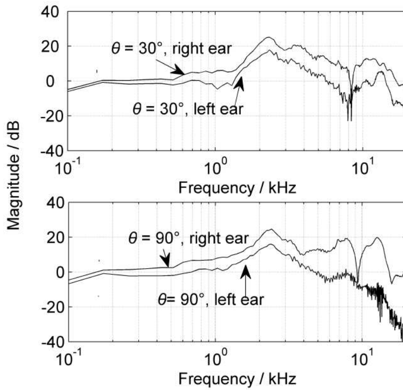
Figure 7. Magnitudes of KEMAR HRTFs at azimuths of 30^\circ and 90^\circ in the horizontal plane
