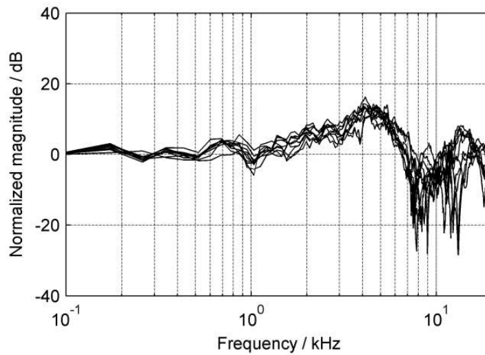
Figure 8. Left-ear HRTF magnitudes for 10 subjects at azimuth 0^\circ in the horizontal plane
