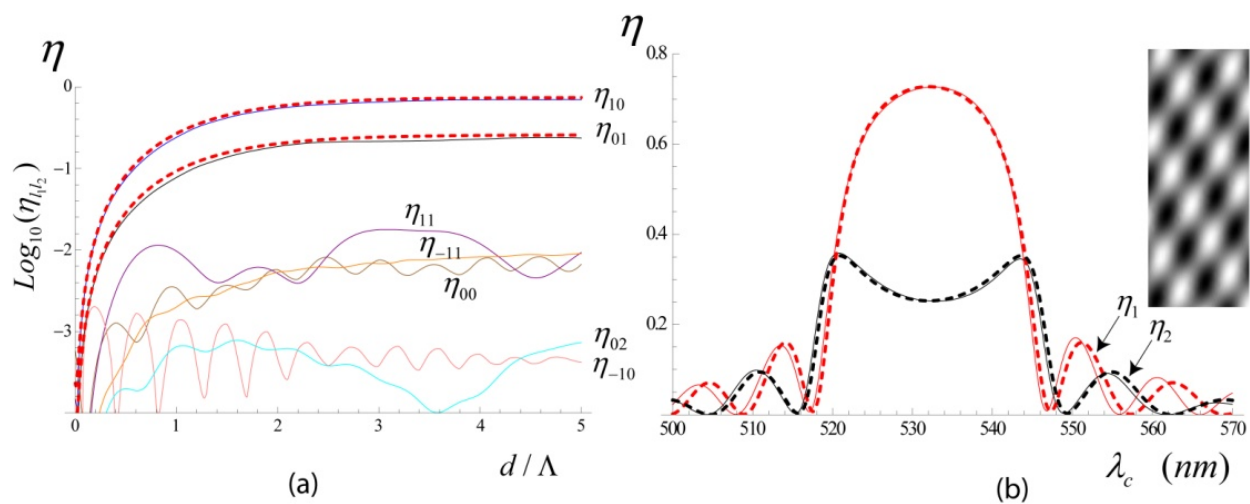
Figure 6. (a) Diffractive Efficiency, \eta_\sigma versus normalised grating thickness, d/\Lambda as predicted by the N-PSM model and by a rigorous coupled wave calculation (RCW) for the case of a twin multiplexed (duplex) reflection grating at Bragg resonance (grating shown in inset photo). The grating is replayed using light of 532nm at an incidence angle of \Phi_c=30^\circ . The grating index modulation of each of the component twin gratings in the duplex has been taken to be n_1=0.2 . The dotted lines indicate the S_1 and S_2 modes of the N-PSM model and the full lines indicate the modes of the RCW calculation. The most prominent RCW modes are the 01 and 10 modes which correspond to the S_1 and S_2 modes in N-PSM. The duplex grating has been recorded with a reference beam angle of \Phi_c=30^\circ and with a wavelength of 532nm. One grating in the duplex has a slope of \psi_1=20^\circ and the other has a slope of \psi_2=-20^\circ . Note that \Lambda refers to the larger of the two grating periods. (b) Diffractive Efficiency, \eta_\sigma versus replay wavelength, \lambda_c as predicted by the N-PSM model and by a RCW calculation for the same duplex grating as used in (a) at and away from Bragg resonance. The grating is again illuminated at its recording angle of \Phi_c=30^\circ . A grating index modulation of n_1=0.03 for each component grating is assumed and a grating thickness of d=7\mu\text{m} is used. The dotted lines indicate the S_1 and S_2 modes of the N-PSM model and the full lines indicate the corresponding 10 and 01 modes of the rigorous coupled wave calculation. In both (a) and (b) the average index inside and outside the grating is n_0=1.5 .
