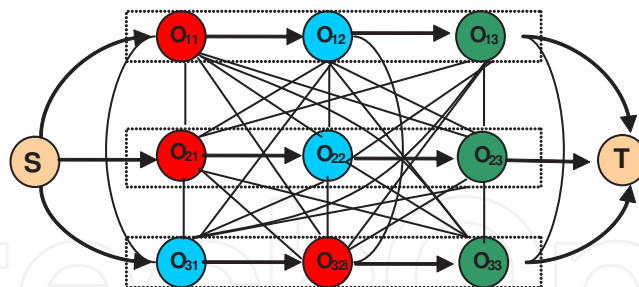
Figure 2. Problem routing representation.
