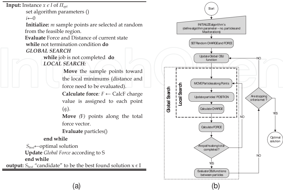
Figure 6. The Electromagnetic like Method; 6a. the EM pseudo code; 6b. the flow chart of a general EM procedure.
