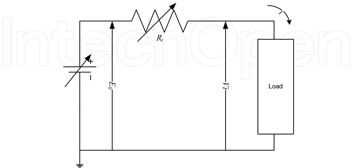
Figure 4. Equivalent electrical circuit of a steady-state battery
