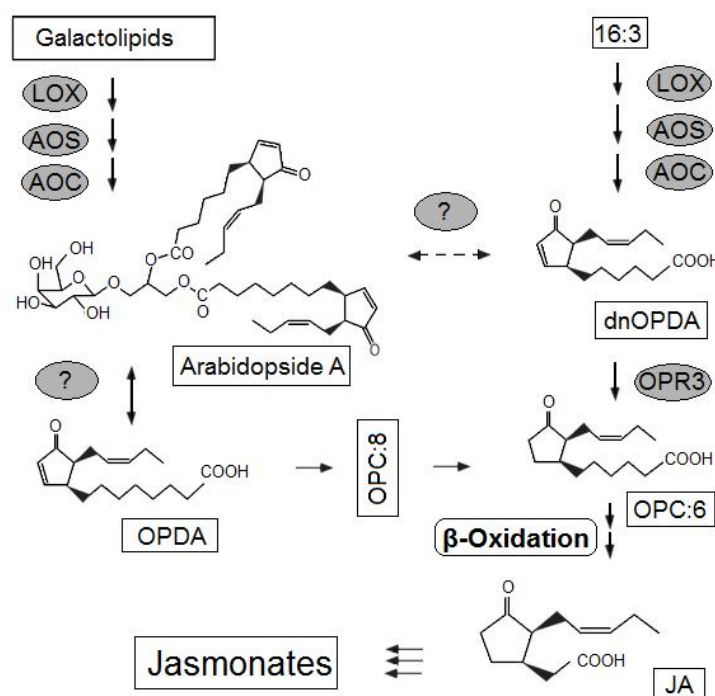
Figure 3. Alternative JA biosynthesis pathway (Schaller et al., 2004; Gfeller et al., 2010)
