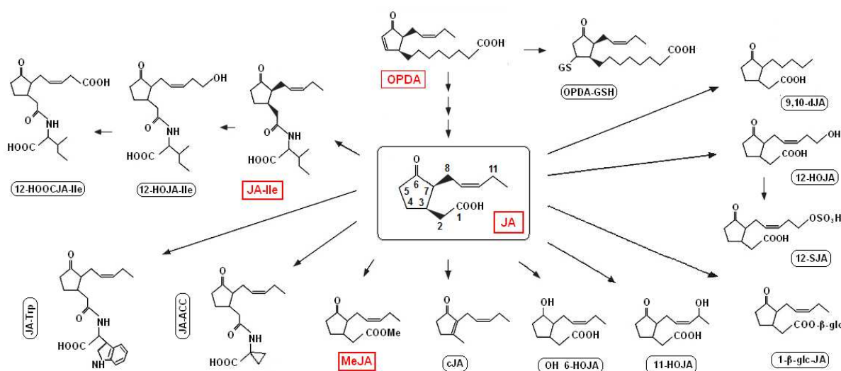
Figure 5. The metabolites produced from JA in plants (Gfeller et al., 2010)
