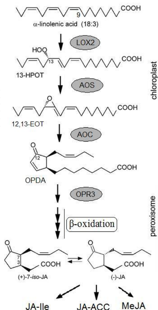
Figure 2. Scheme of JA biosynthesis pathway in A. thaliana (Delker et al., 2006)
