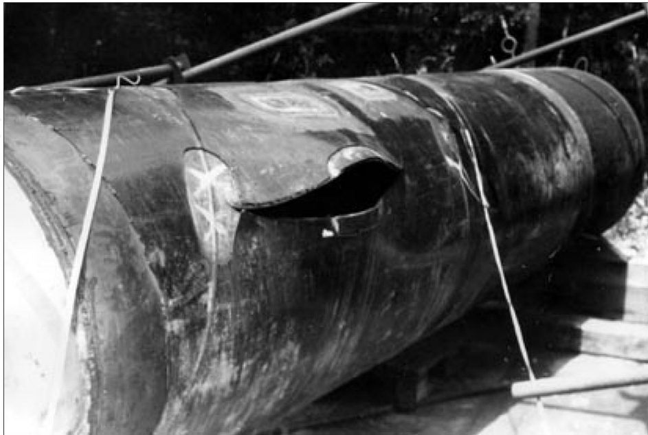
Figure 16. Burst initiated on slit B with a fatigue crack
