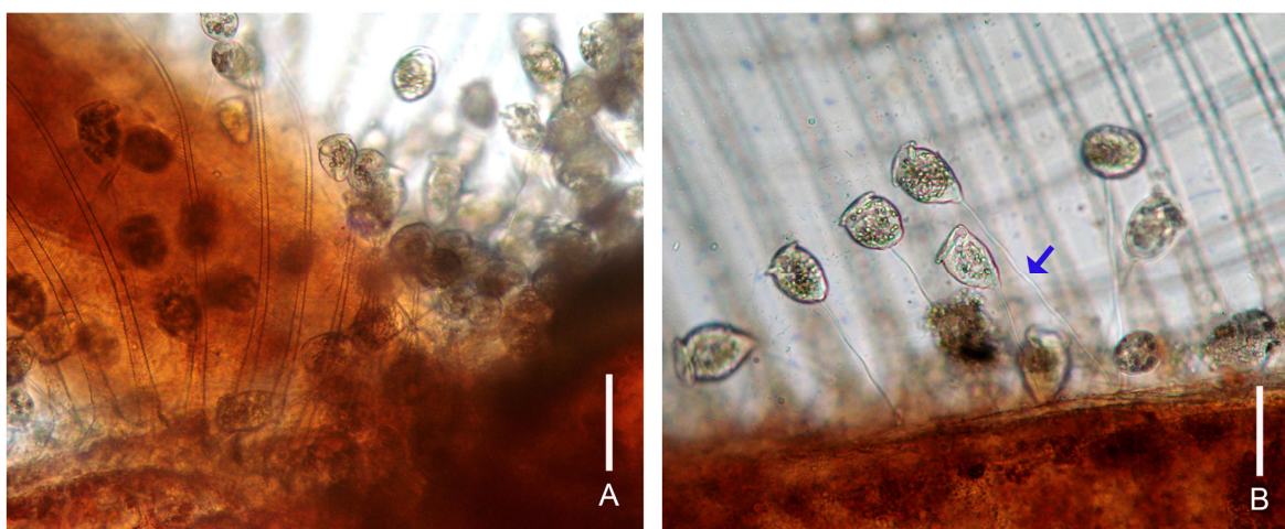
Figure 2. Vorticella sp.
