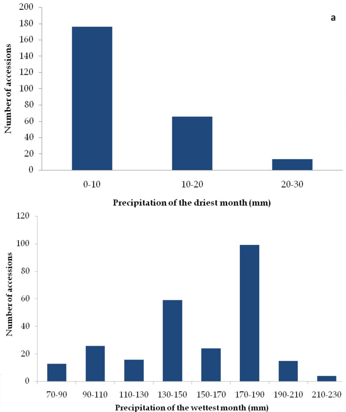
Figure 8. Groupings of target plants based on GIS-derived ecological criteria: Number of accession numbers of target plants (n=256) originating from the Aegean Archipelago, the Ionian Islands, Crete and Peloponnese (Greece) grouped according to precipitation classes during the driest (a) and wettest (b) months of the year. For each class specific plant lists can also be generated.
