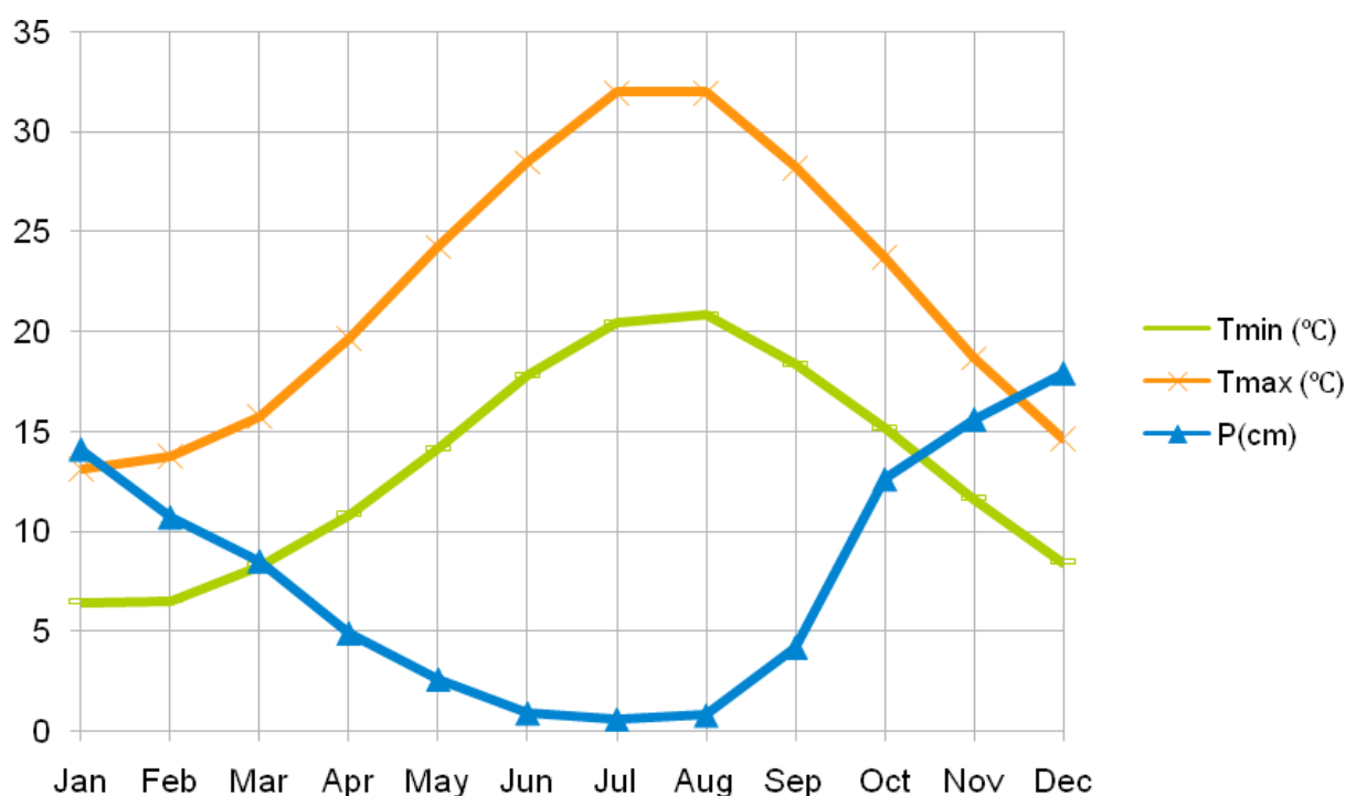
Figure 5. Monthly variations of the climatic conditions (average values of 50 years for precipitation, minimum and maximum temperature) at the original collection sites of Silene cephallenia subsp. cephallenia derived from its ecological fact sheet.
