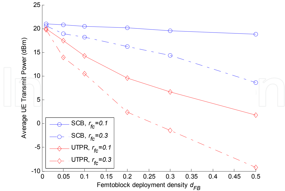
Figure 5. Average UE transmit power versus the d_{FB}
