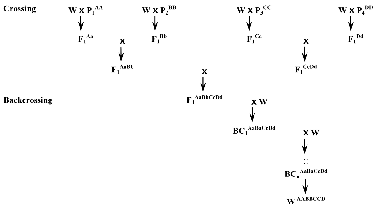
Scheme 2. Simultaneous/Synchronized Backcrossing
