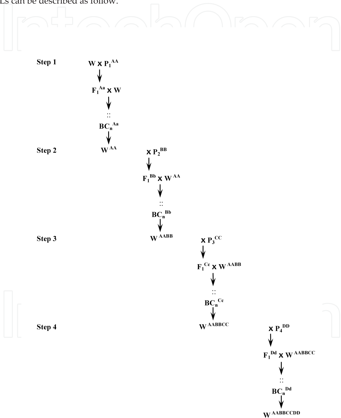
Scheme 1. Stepwise Backcrossing
