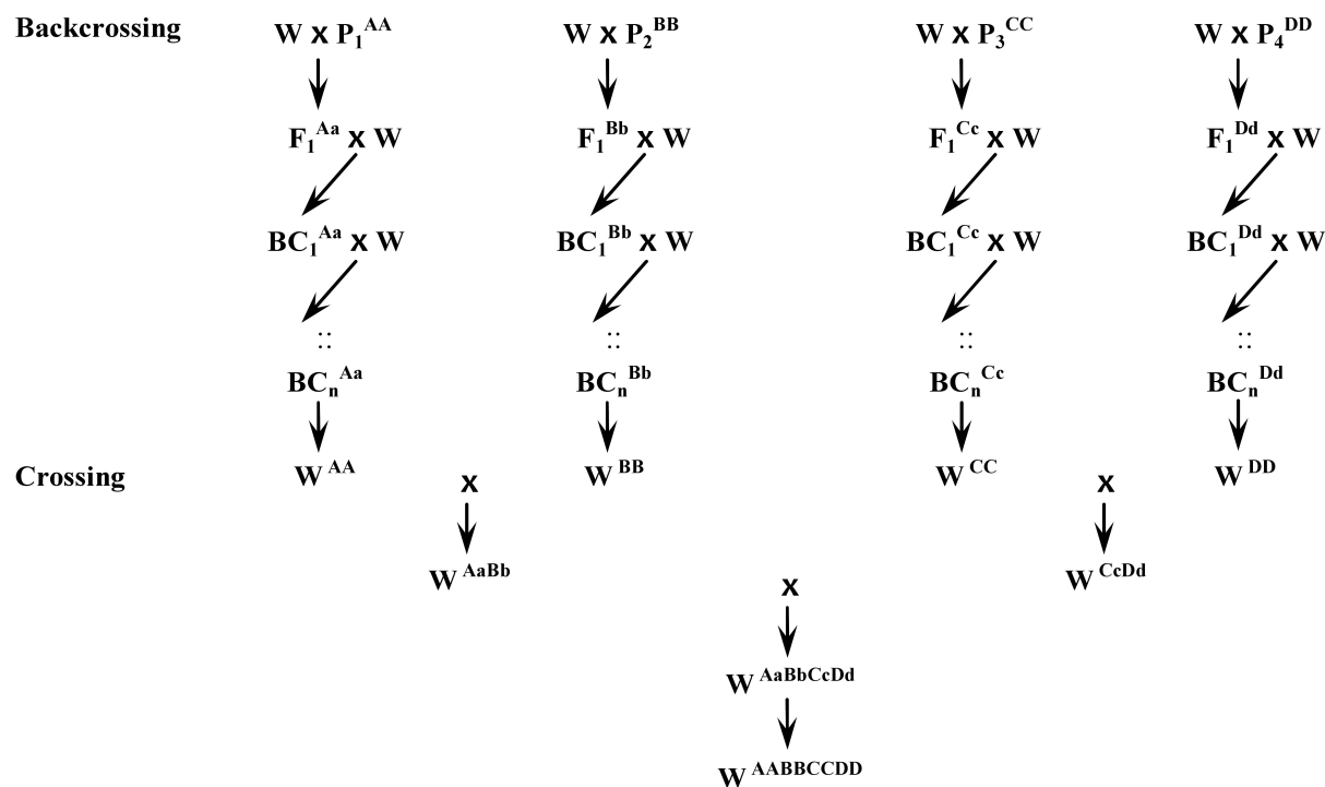
Scheme 3. Convergent Backcrossing
