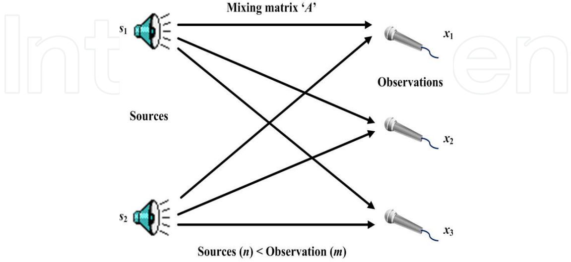
Fig. 10. Illustration of “undercomplete ICA”
