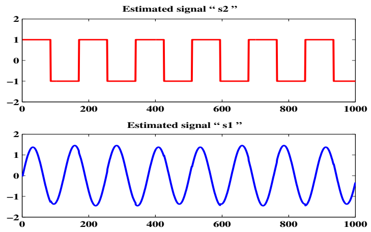
Fig. 4. Estimates of independent components
