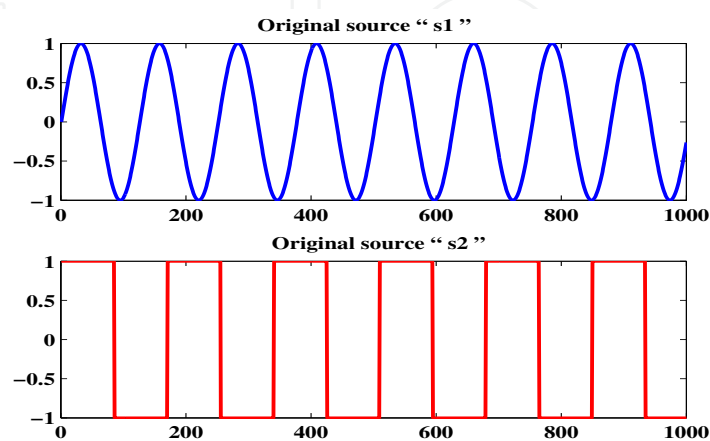
Fig. 2. Independent sources s_1 and s_2
