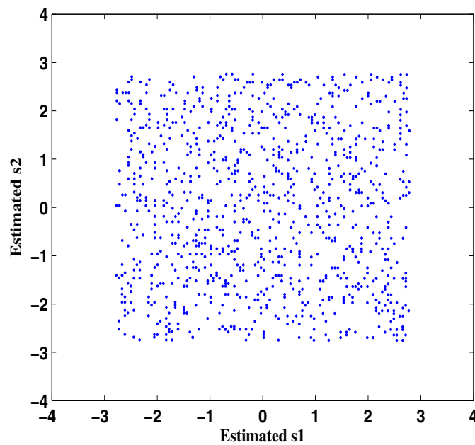
Fig. 8. ICA solution (Estimated sources)
