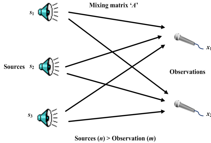
Fig. 9. Illustration of “overcomplete ICA”
