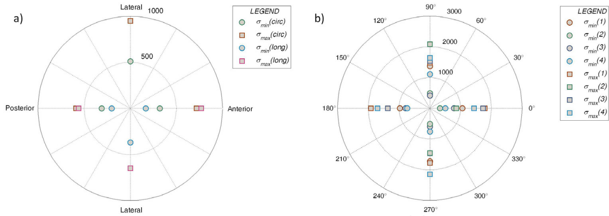
Figure 6. Yield stress in circumferential (upper side) and longitudinal (lower side) direction from [70] (a). Failure stress by circumferential location as anterior (0°), left (90°), posterior (180°) and right (270°) regions from [54] (b).
