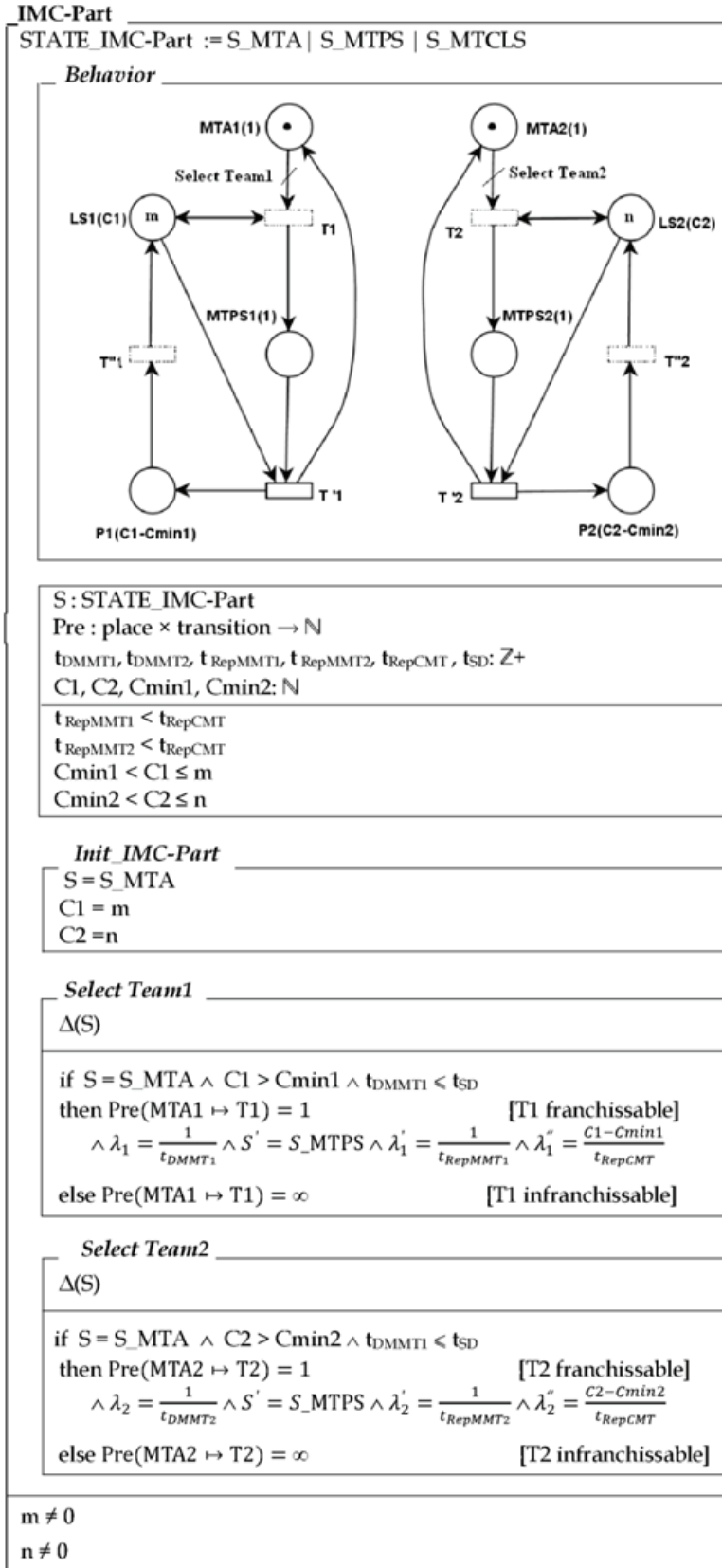
Figure 13. IMC-Part system specification based on SPNOZ syntax
