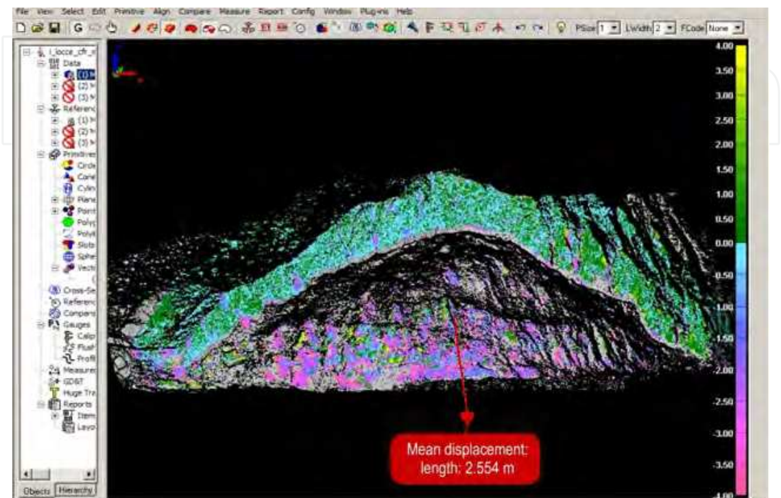
Fig. 12. Map of landslide collapse computed by subtracting the two multitemporal surfaces along the average displacement vector
