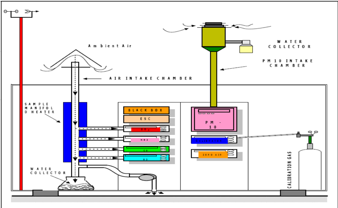
Fig. 3. Schematic Diagram of CAQM (Source: DOE, 2008).
