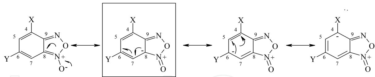
Scheme 2. Resonance forms of substituted benzofuroxans.
