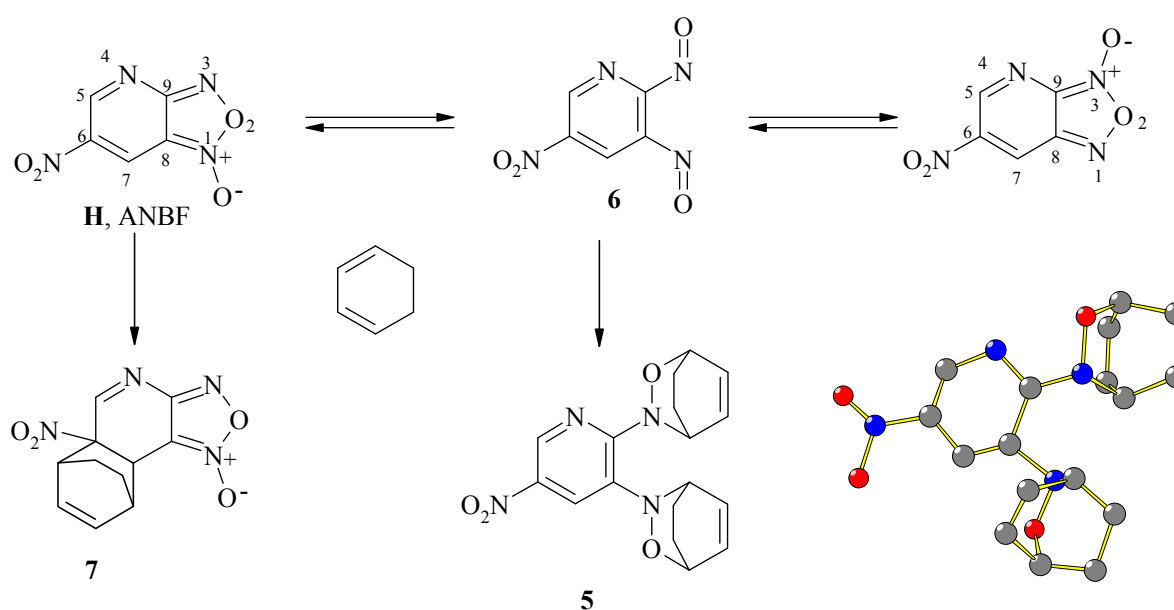
Scheme 1. Diels-Alder Trapping of the o -dinitroso intermediate 6 .
