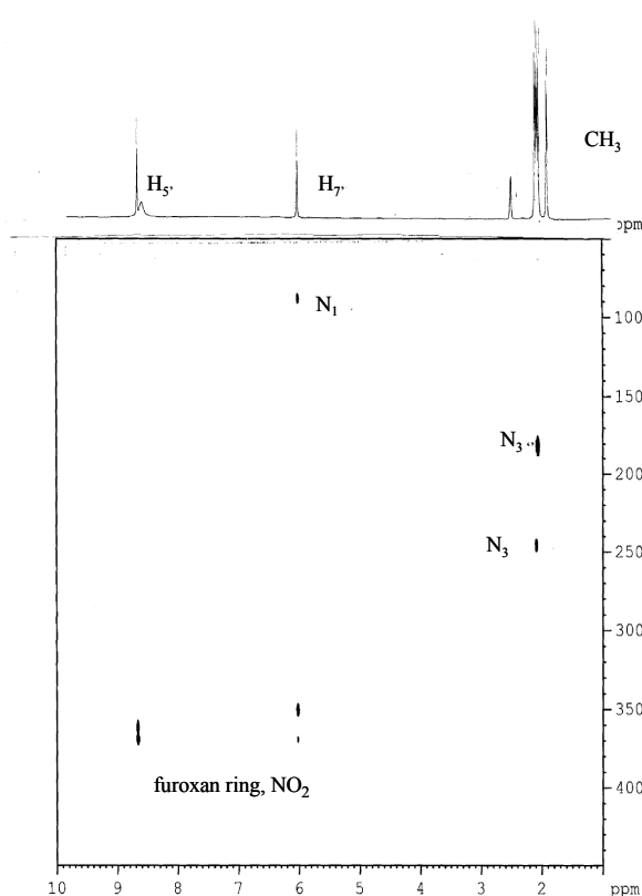
Fig. 4a. ^1\text{H} - ^{15}\text{N} correlation for the adduct N-30;30,H ^+
