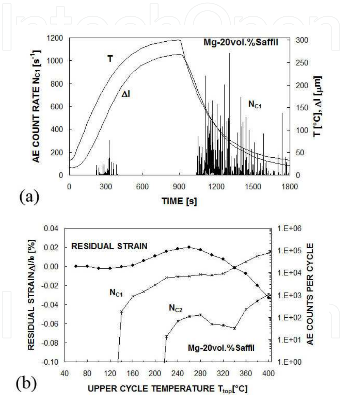
Fig. 10. (a) Value of the AE count rate 1, temperature and sample deformation ( \Delta l ) during temperature cycles to upper temperature of 300 ^{\circ}C . (b) Residual strain, \Delta l / l_0 , and AE counts for two different detection levels, N_{C1} and N_{C2} , versus the upper cycling temperature, T_{top} : the residual strain was estimated with reference to a temperature of 30 ^{\circ}C and the AE counts were evaluated for the entire cooling period of each cycle.
