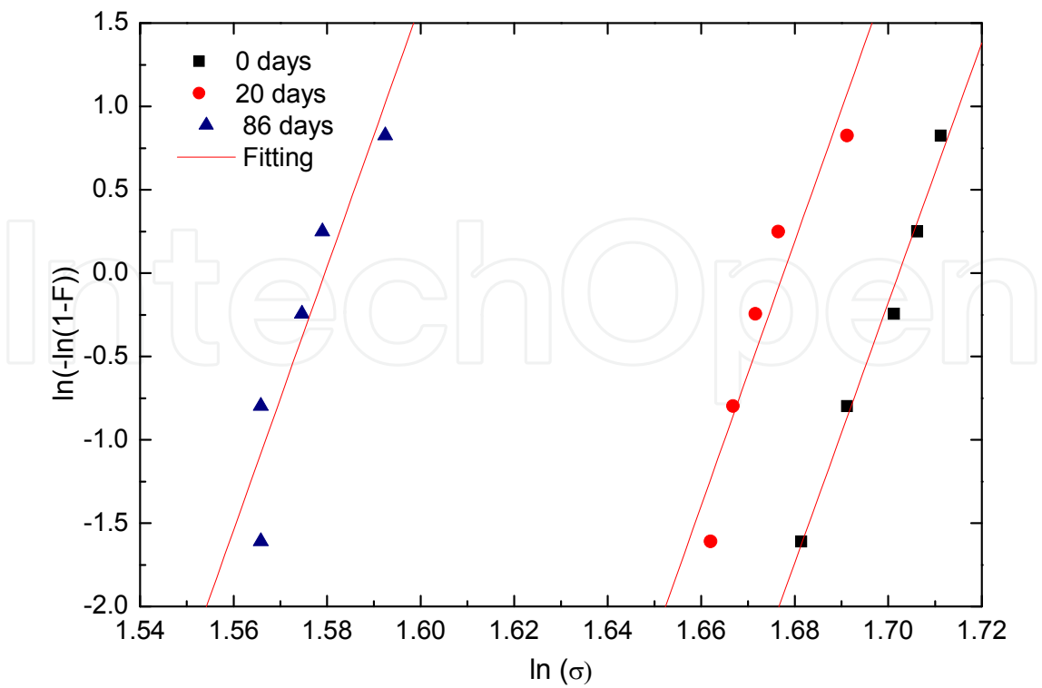
Fig. 9. Cumulative failure probability for fibers aged in the same NaCl concentration for different periods of time.
