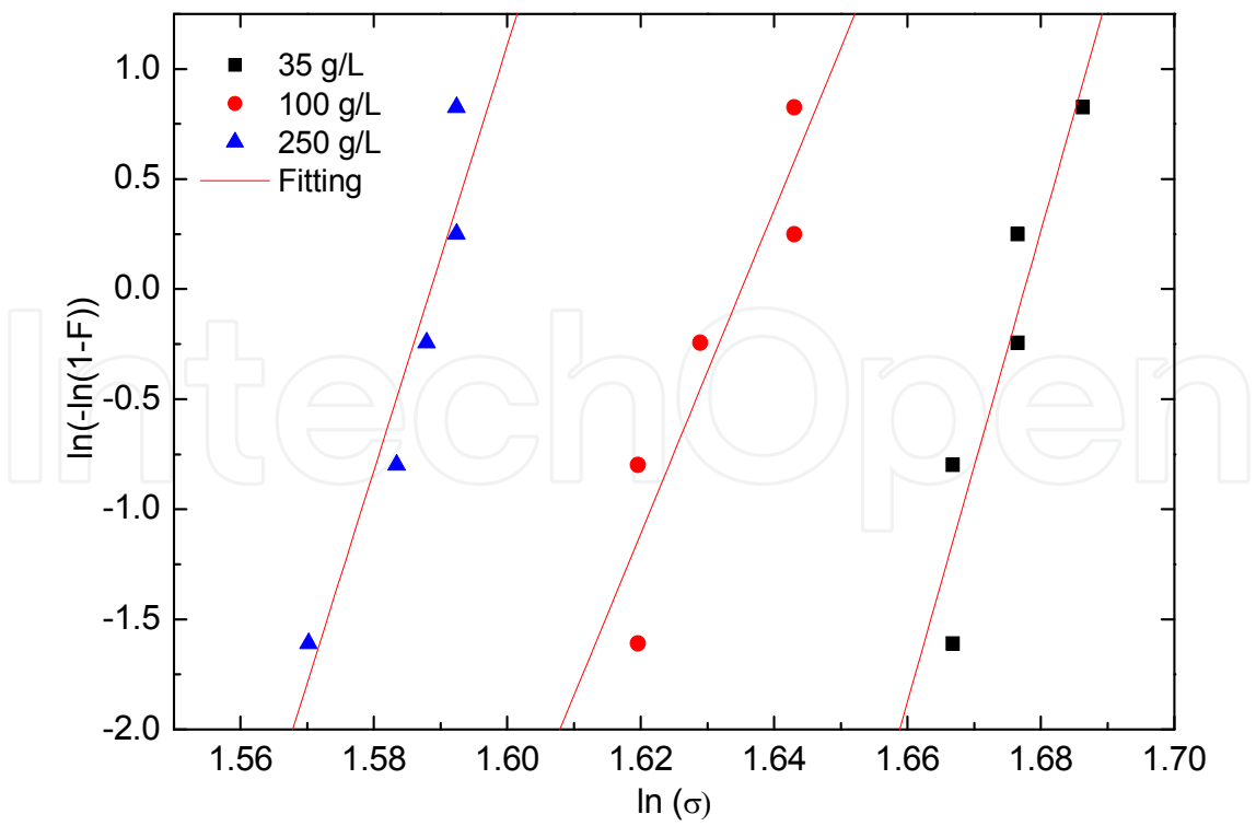
Fig. 10. Cumulative failure probability for fibers aged in different NaCl concentrations for the same period of time.
