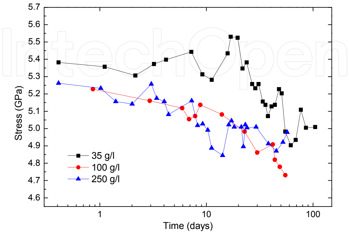
Fig. 6. Fracture stress values along degradation time for the fibers aged in the 35, 100 and 250 g/L NaCl solutions.
