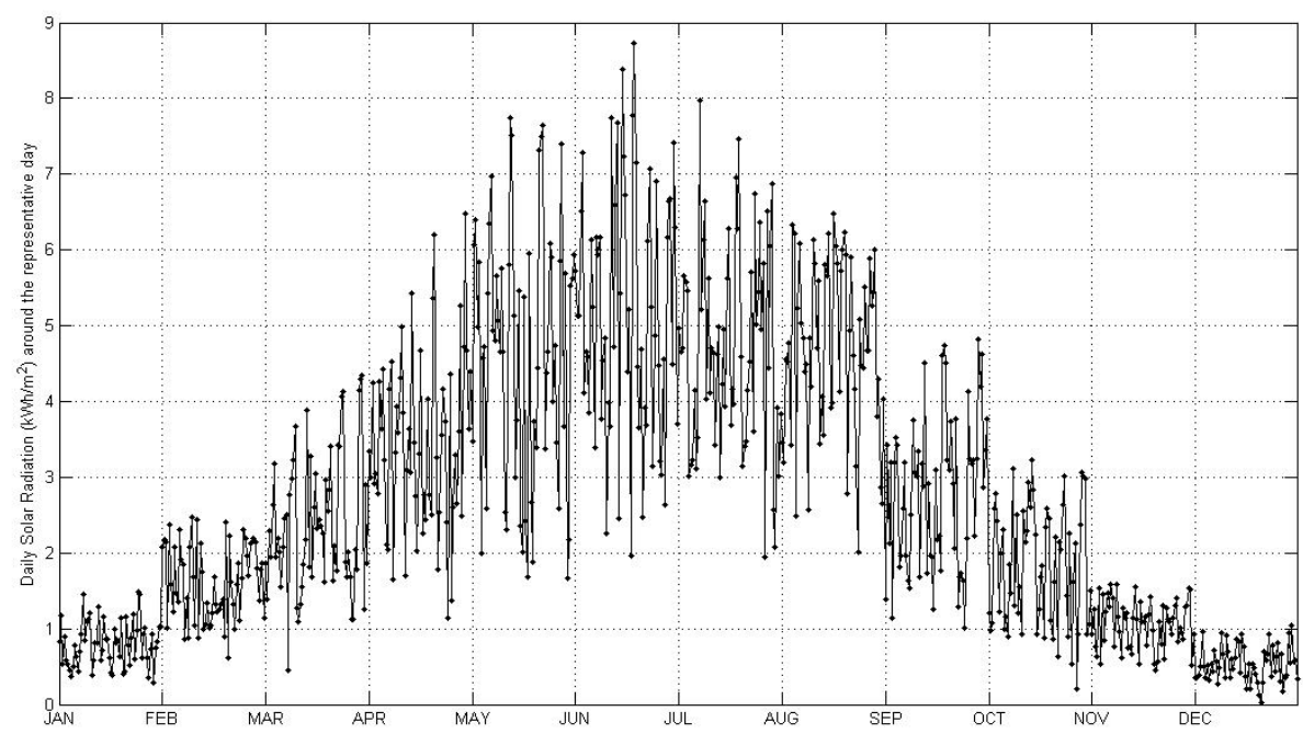
Fig. 4. Daily solar radiation (kWh/m²) around the representative day of each month for the 20 year period (1985-2004), in the city of London, UK.
