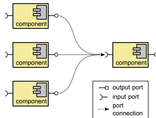
Fig. 3. Port connections: many publishers, one subscriber.
