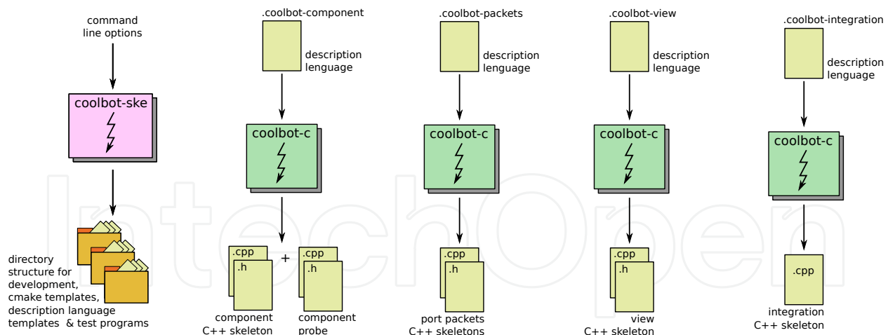
Fig. 6. CoolBOT's software development process.
