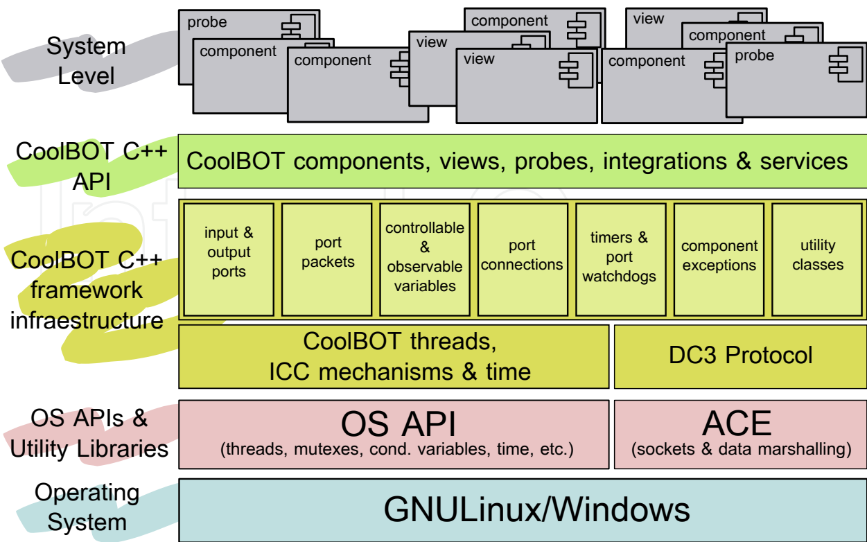
Fig. 5. Abstraction layers in CoolBOT.
