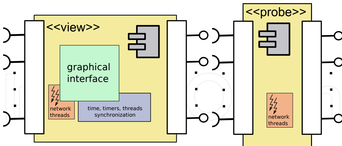
Fig. 7. CoolBOT. View and probe structures.
