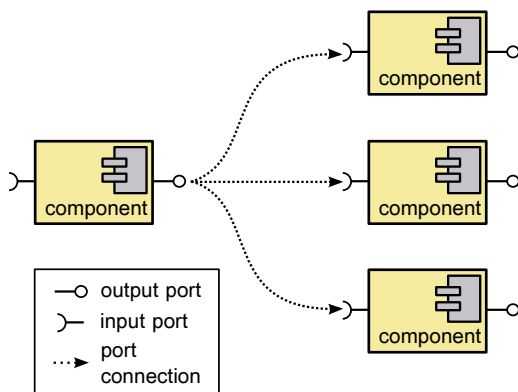
Fig. 2. Port connections: one publisher, many subscribers.
