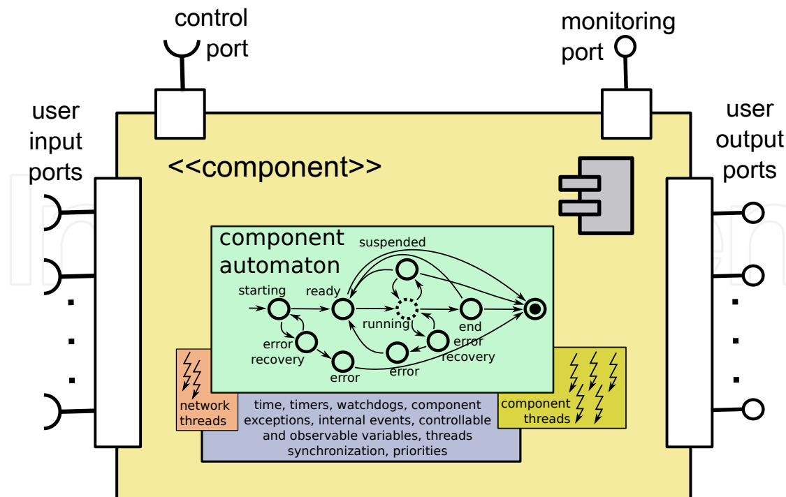
Fig. 4. CoolBOT. Component structure.
