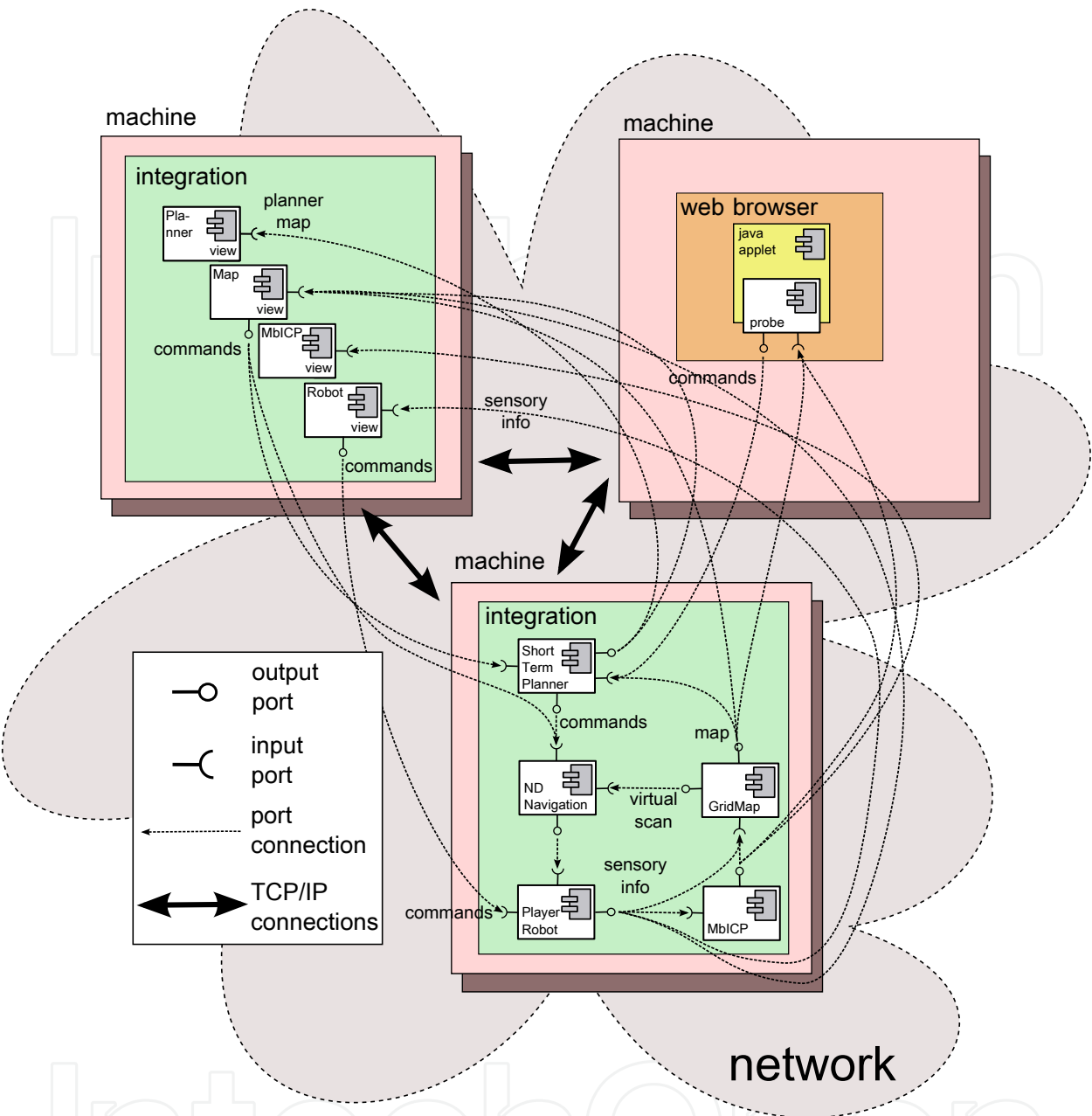
Fig. 8. CoolBOT. Secure Navigation System.
